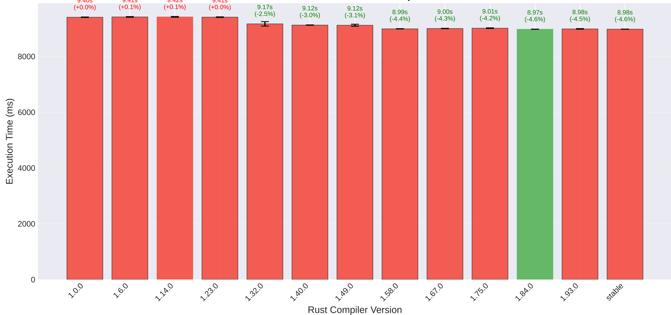
Execution Time Across Rust Compiler Versions
