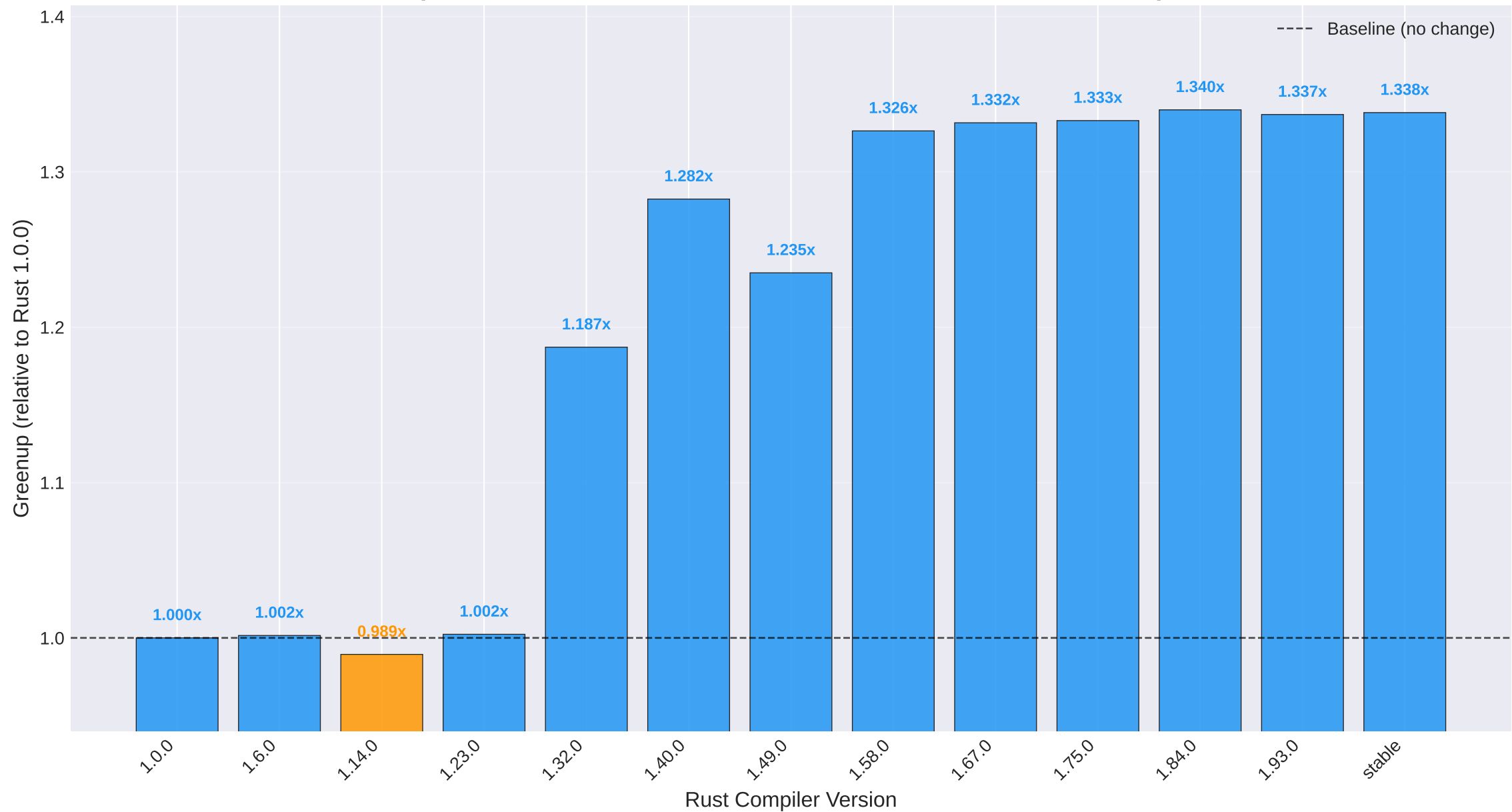
Greenup (Energy Efficiency) Across Rust Compiler Versions (Baseline: Rust 1.0.0, >1.0 = more efficient, <1.0 = less efficient)
