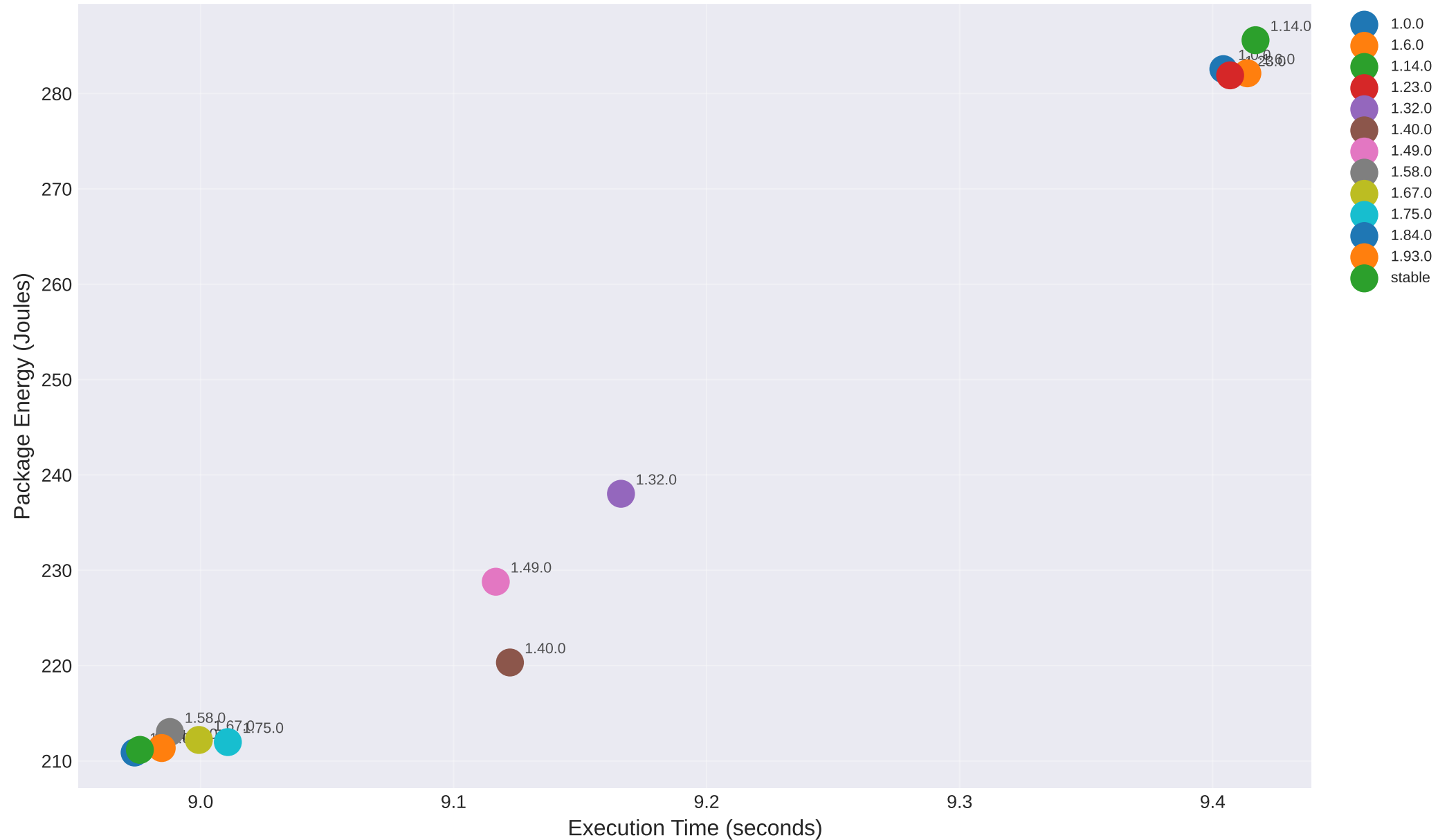
Performance per Watt: Energy vs Time Across Rust Versions (Lower and further left = better)
