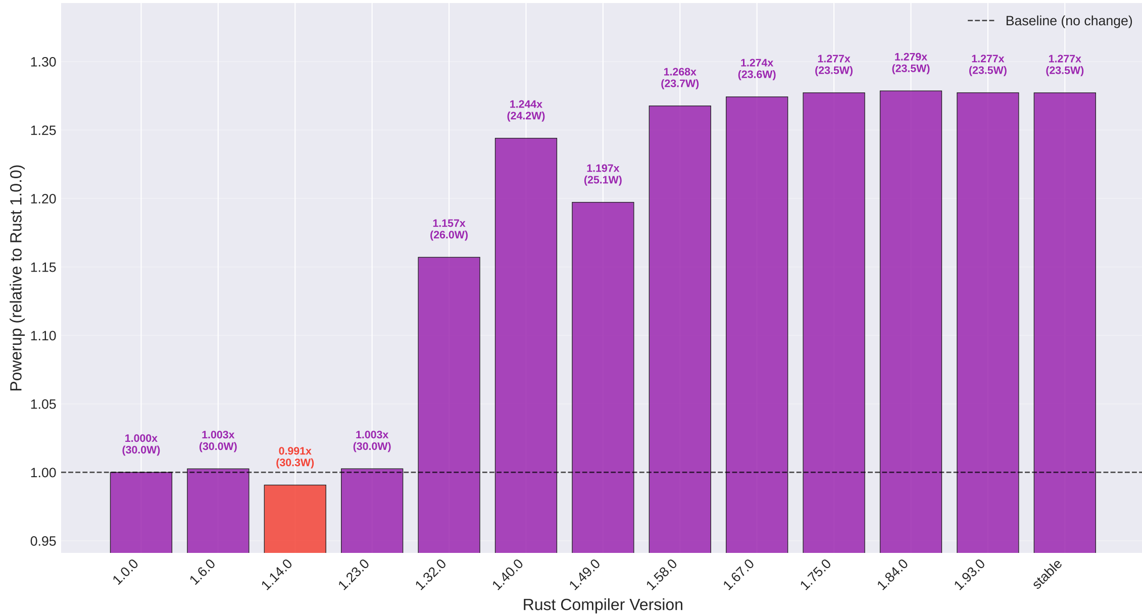
Powerup (Average Power Efficiency) Across Rust Compiler Versions (Baseline: Rust 1.0.0, >1.0 = lower avg power, <1.0 = higher avg power)
