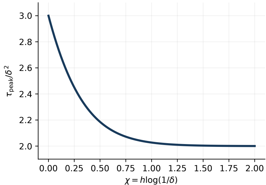
Peak location in the joint limit
