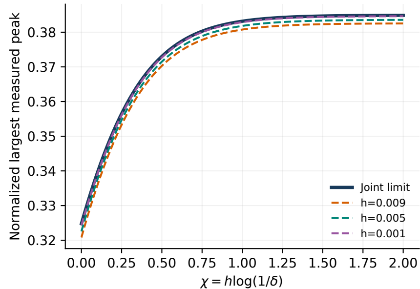
A slow anisotropy crossover
