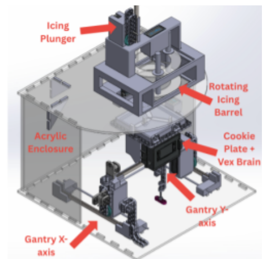
CAD of Overall Layout
