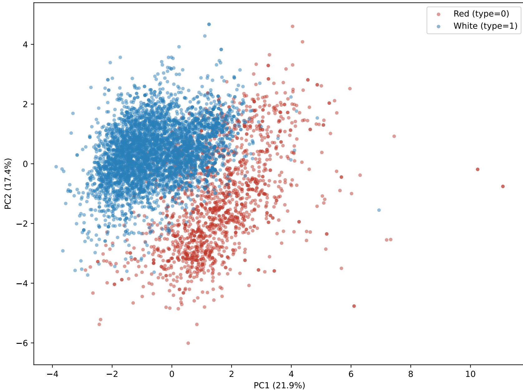
PCA of Wine Data — Colored by Type (Red vs White)
