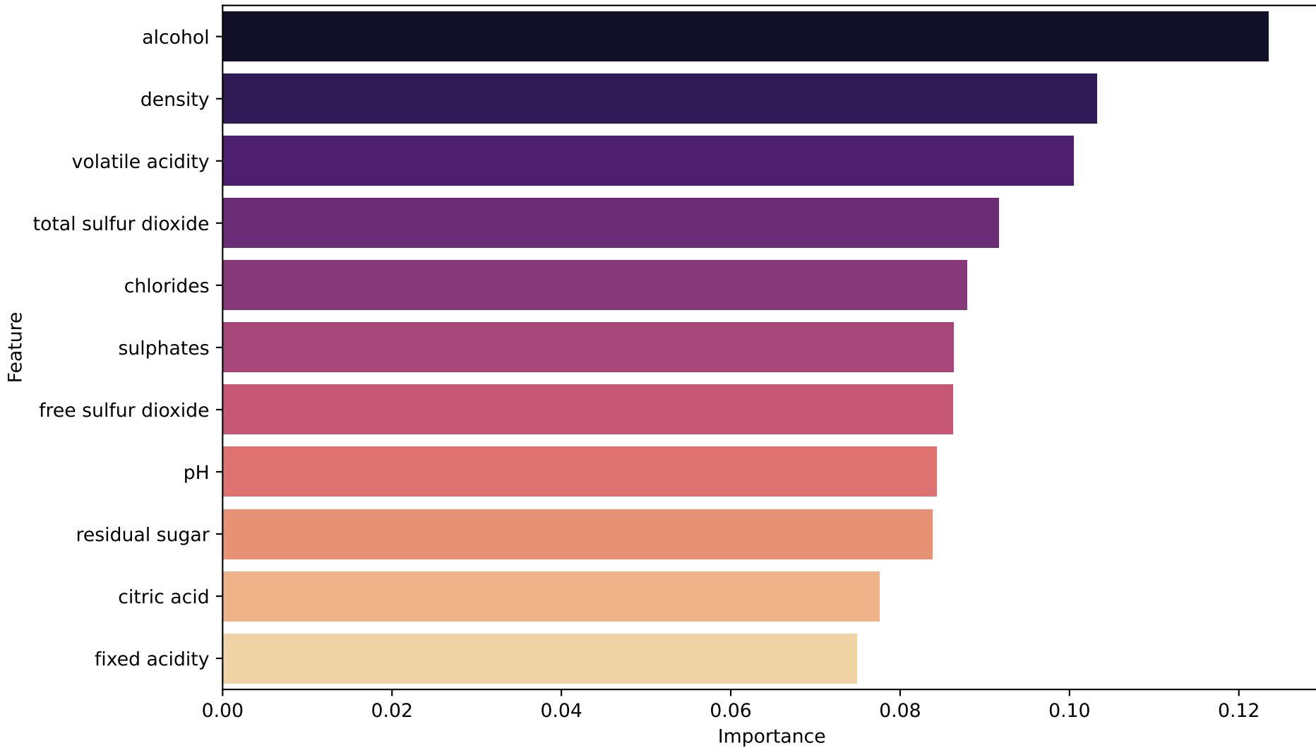
Feature Importance for Predicting Quality (Random Forest)
