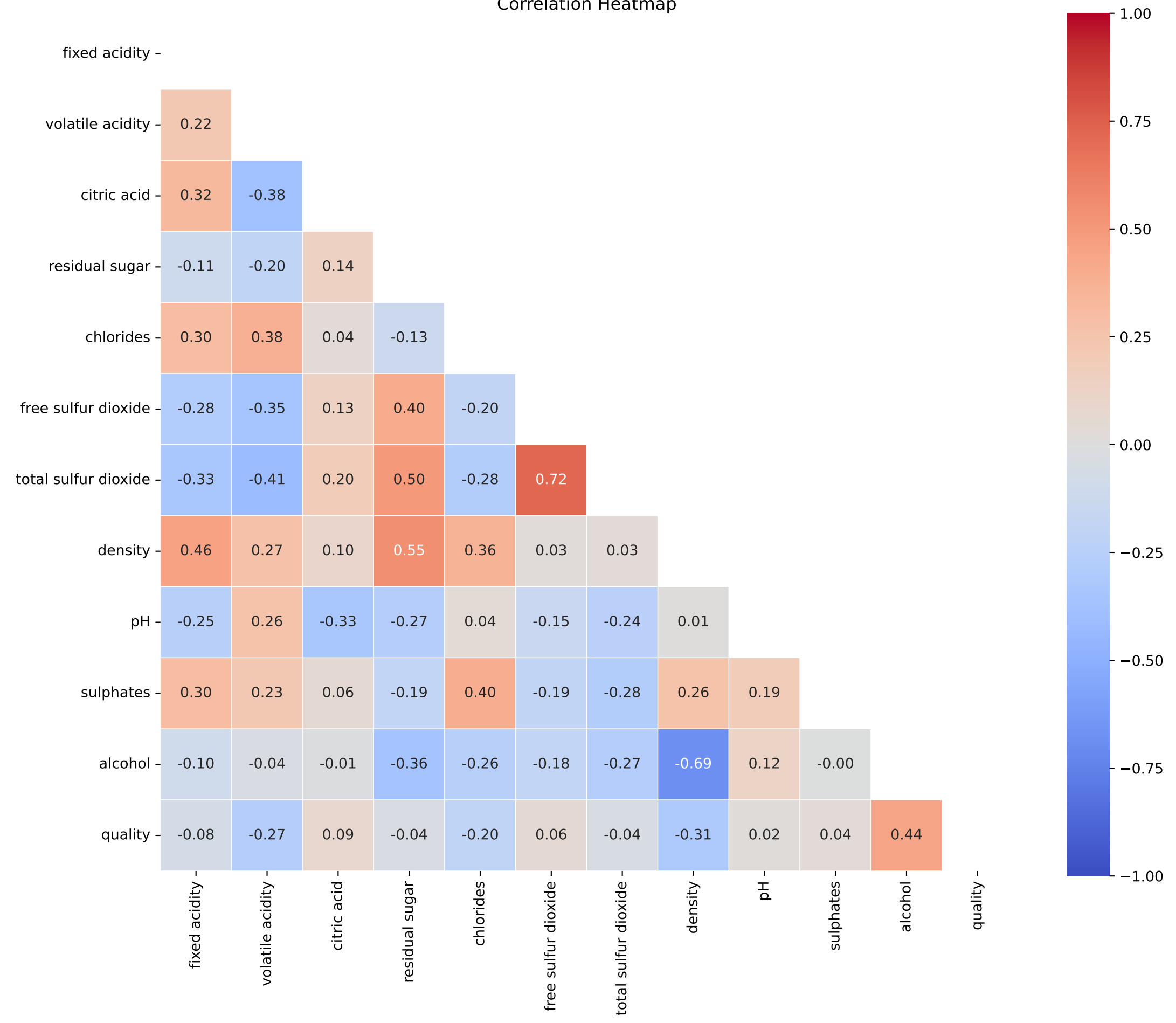
Correlation Heatmap
