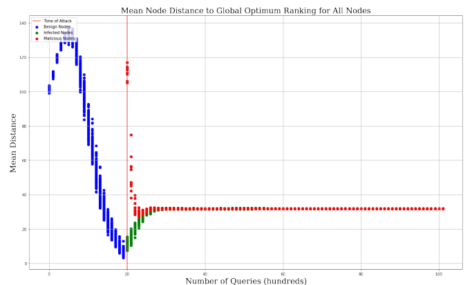
Fig. 3. Targeted Sybil Attack: The mean distance to the optimal ranking for each node, across all possible query terms.
