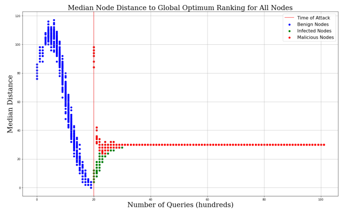
Fig. 2. Targeted Sybil Attack: The median distance to the optimal ranking for each node, across all possible query terms. Post-attack, non-malicious nodes converge higher towards an equilibrium.
