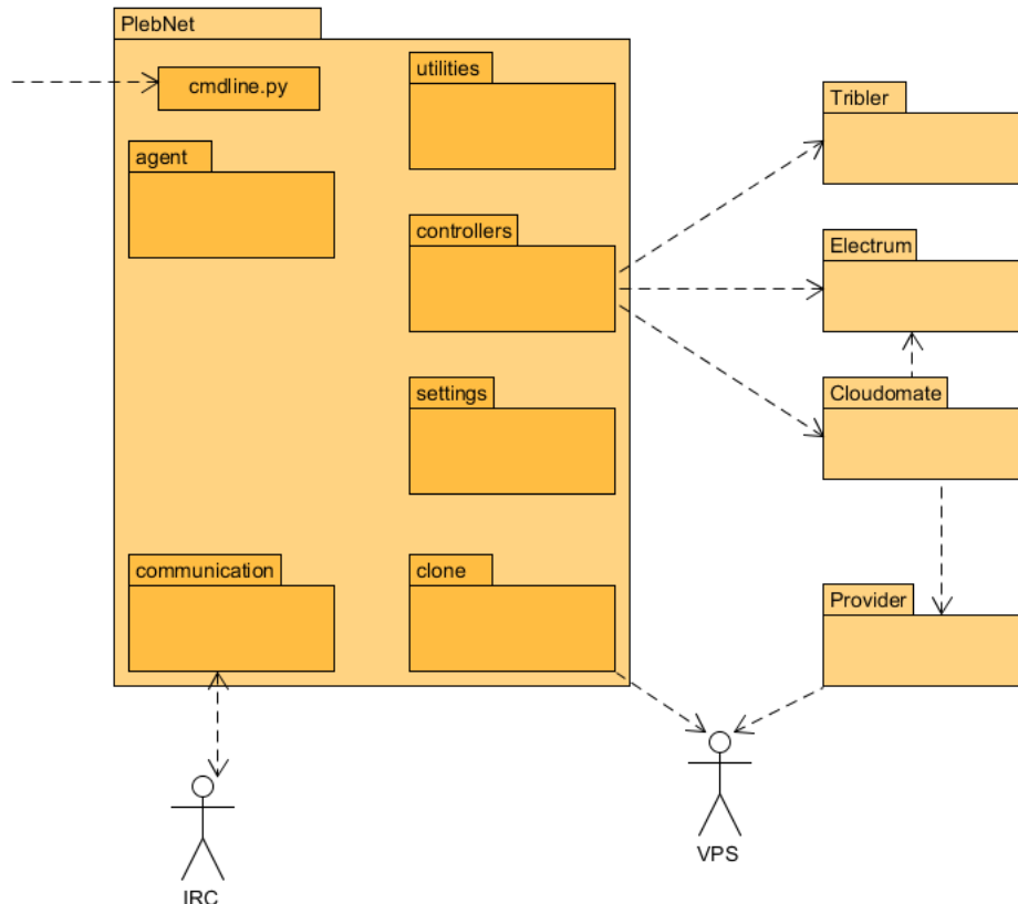
Figure 5.1: Package diagram
