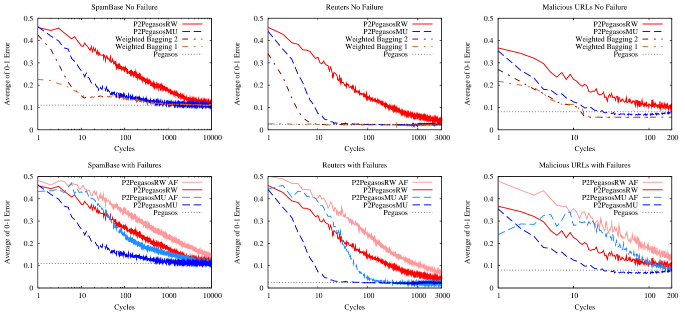
Fig. 1. Experimental results without failure (upper row) and with extreme failure (lower row). AF means all possible failures are modeled.
