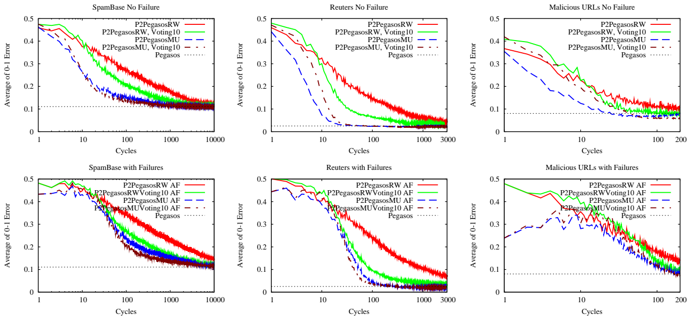
Fig. 3. Experimental results applying local voting without failure (upper row) and with extreme failure (lower row).
