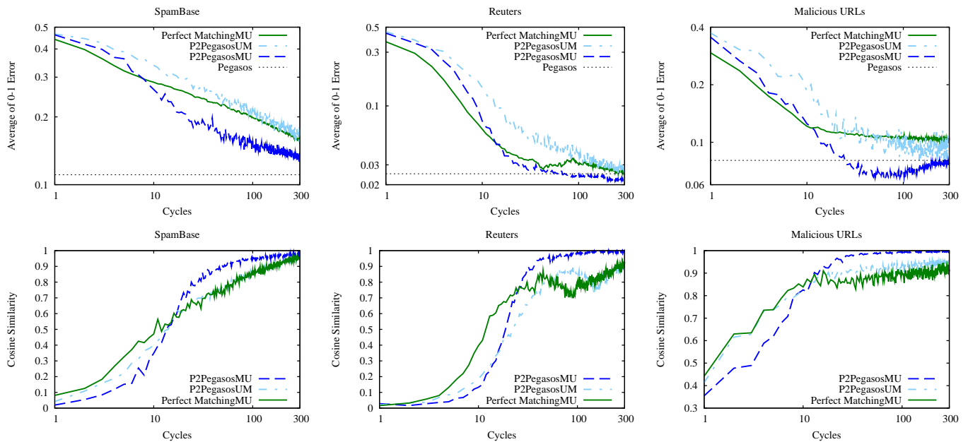
Fig. 2. Prediction error (upper row) and model similarity (lower row) with PERFECT MATCHING and P2PEGASUSUM.
