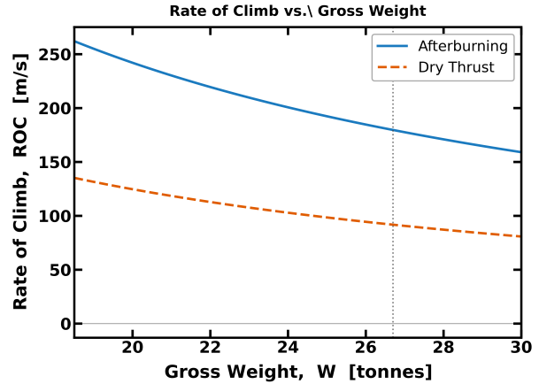
Fig. 9 Rate of climb vs. gross weight.
