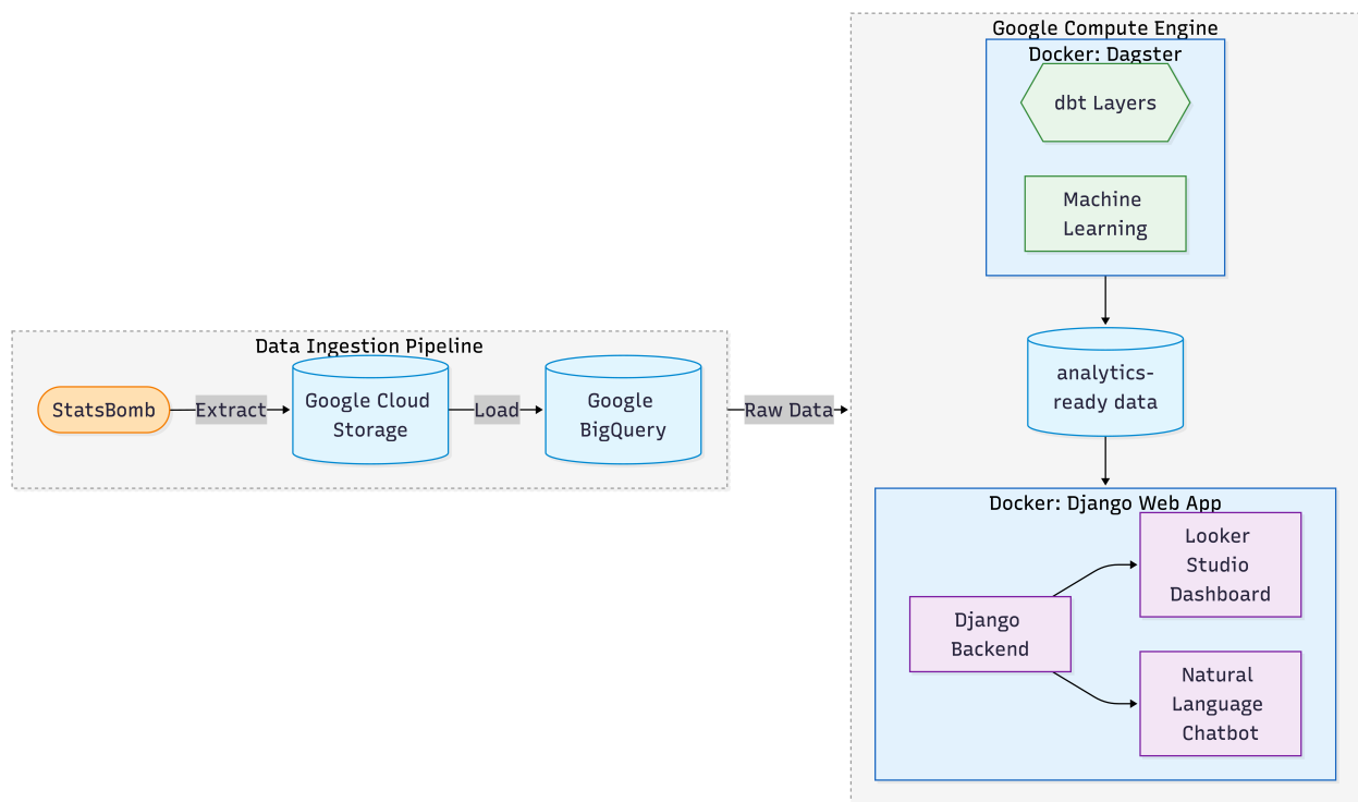
Figure 2: Automated ELT pipeline from StatsBomb open data through BigQuery, dbt, and Python ML scripts to Looker Studio and a Django chatbot, orchestrated by Dagster.
