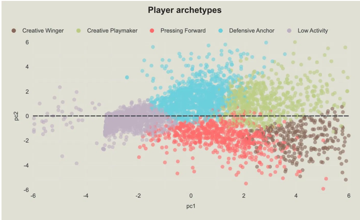
Figure 2: Looker cluster explorer scatter plot of player-seasons in PCA space (PC1 vs PC2), coloured by assigned archetype.
