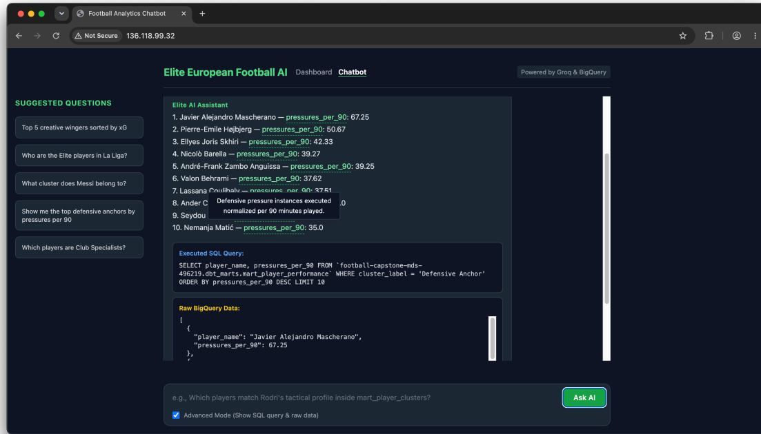
Figure 5: Django chatbot with Advanced Mode enabled, showing a natural language query, generated BigQuery SQL, and formatted results.
