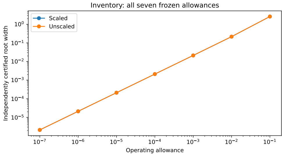
FIGURE 5.—Inventory: every frozen allowance point. These are measured certificate widths, not the exact-LP theorem bound.
