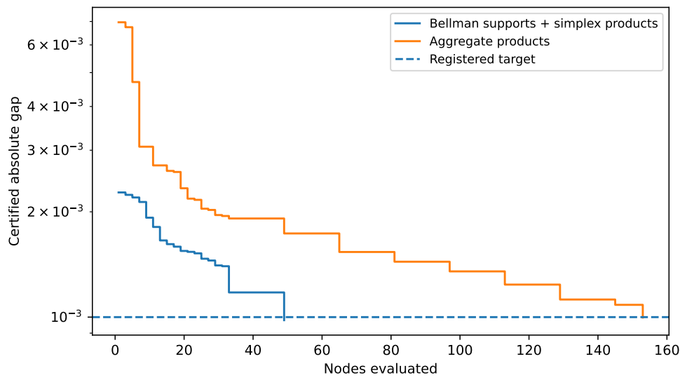
FIGURE 3.—Q1: full-cover certified gap versus nodes. The main article reports the corresponding time trace.
