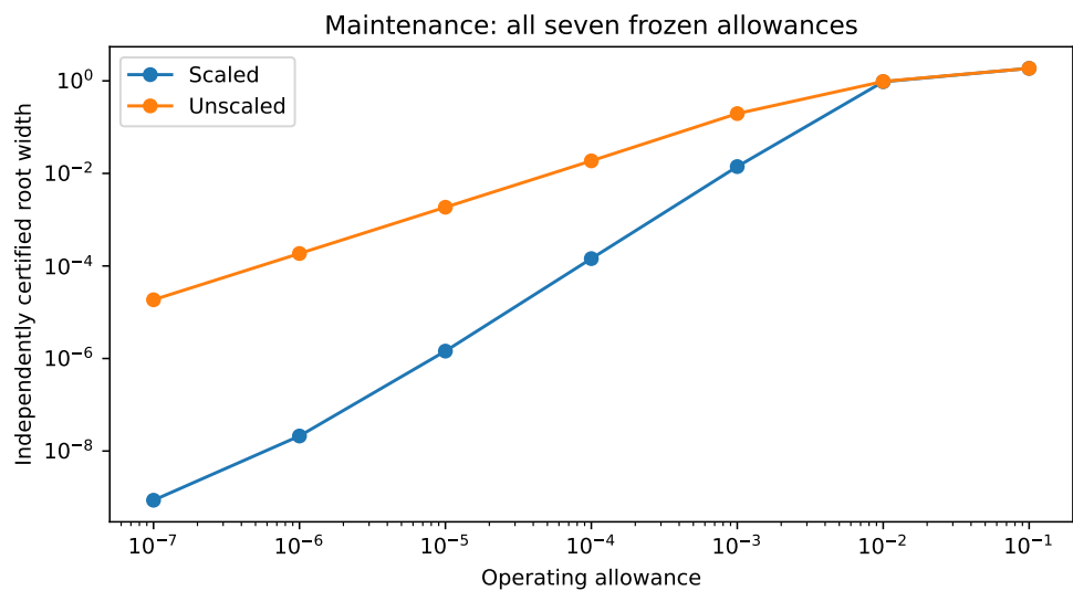
FIGURE 4.—Maintenance: every frozen allowance point. These are measured certificate widths, not the exact-LP theorem bound.
