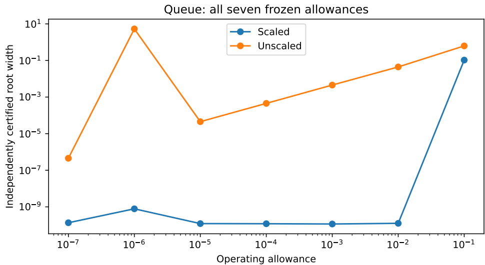
FIGURE 6.—Queue: every frozen allowance point. These are measured certificate widths, not the exact-LP theorem bound.
