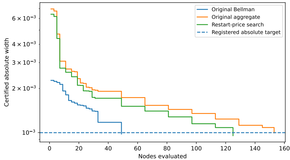
FIGURE 1.—Q1: complete-cover progress by evaluated nodes. Price search reuses an inherited certified incumbent. Nodes across formulations have different costs; this is not an equal-total-work comparison.
