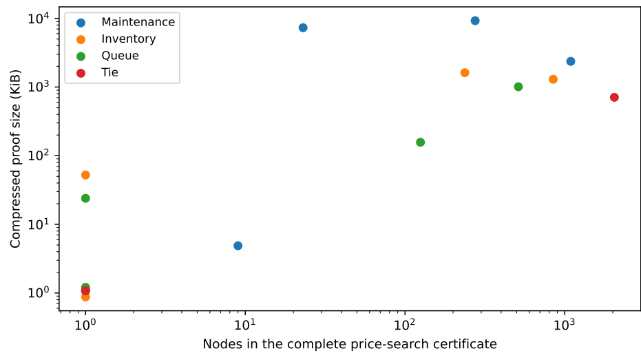
FIGURE 2.—All sixteen retrospective price-search proofs: compressed size versus node count. Each point is an environment, not an independently sampled scaling treatment. Root-only cases remain included.
