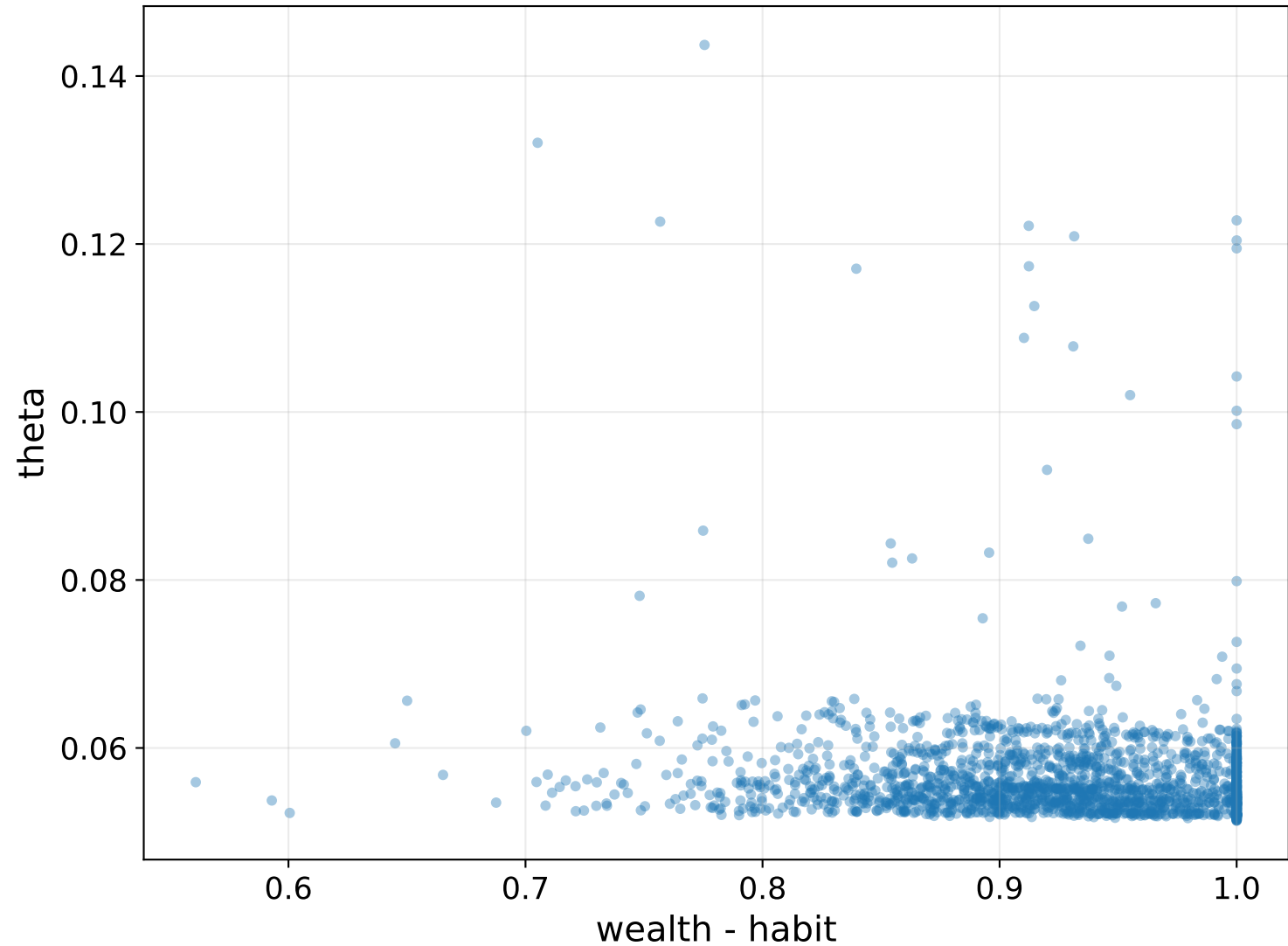
Mechanism diagnostic: theta vs surplus
