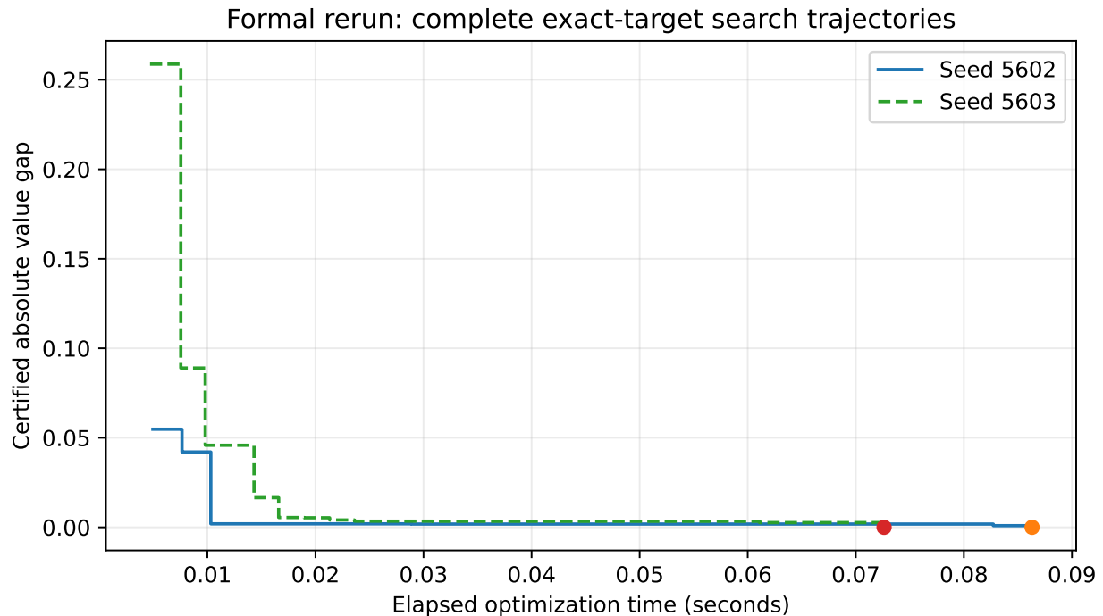
Figure EC.1: Complete recorded exact-target price trajectories for the two eight-history instances requiring branching. Every recorded epoch is retained. The final circles denote zero rational width; elapsed times are those of the published two-second-limit runs, not the later mechanical replay.
