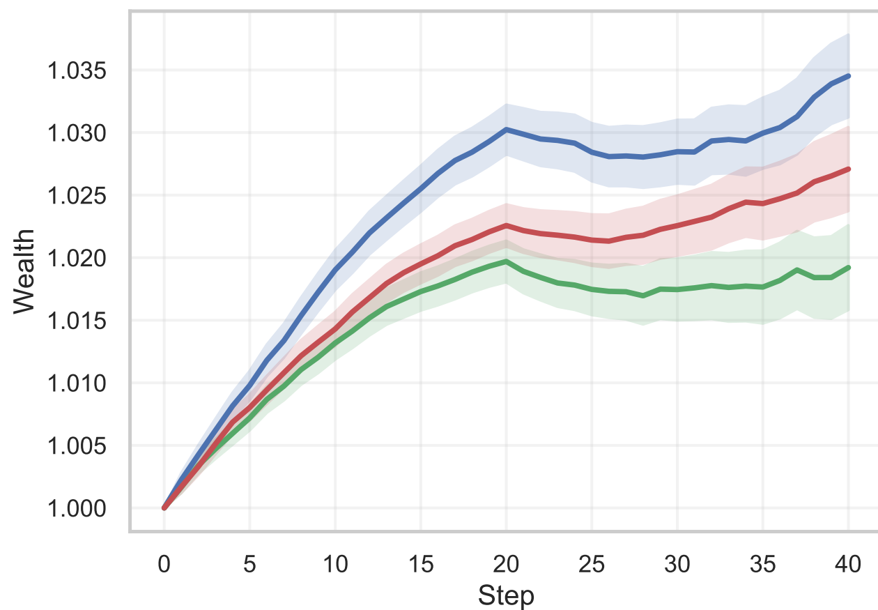
Experiment I: mean wealth path
