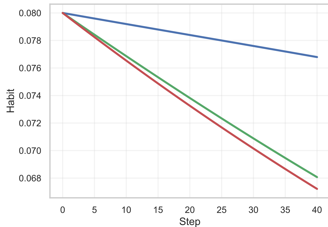
Experiment I: mean habit path
