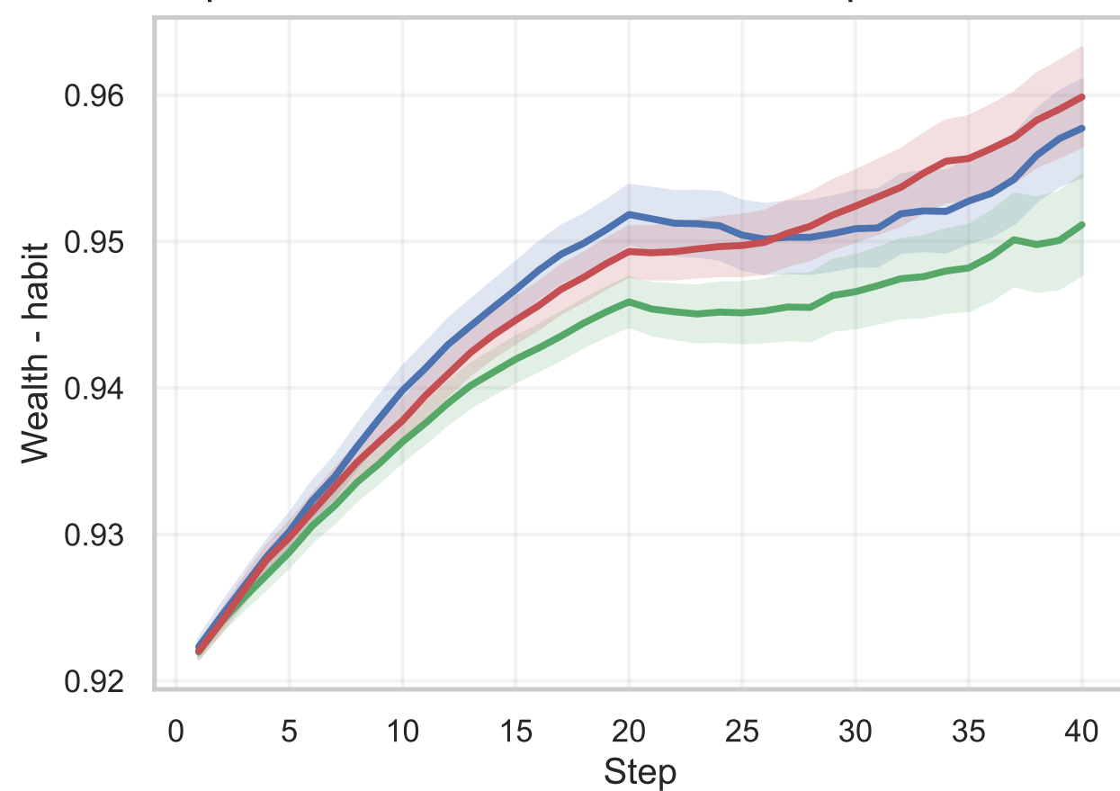
Experiment I: mean wealth-habit surplus
