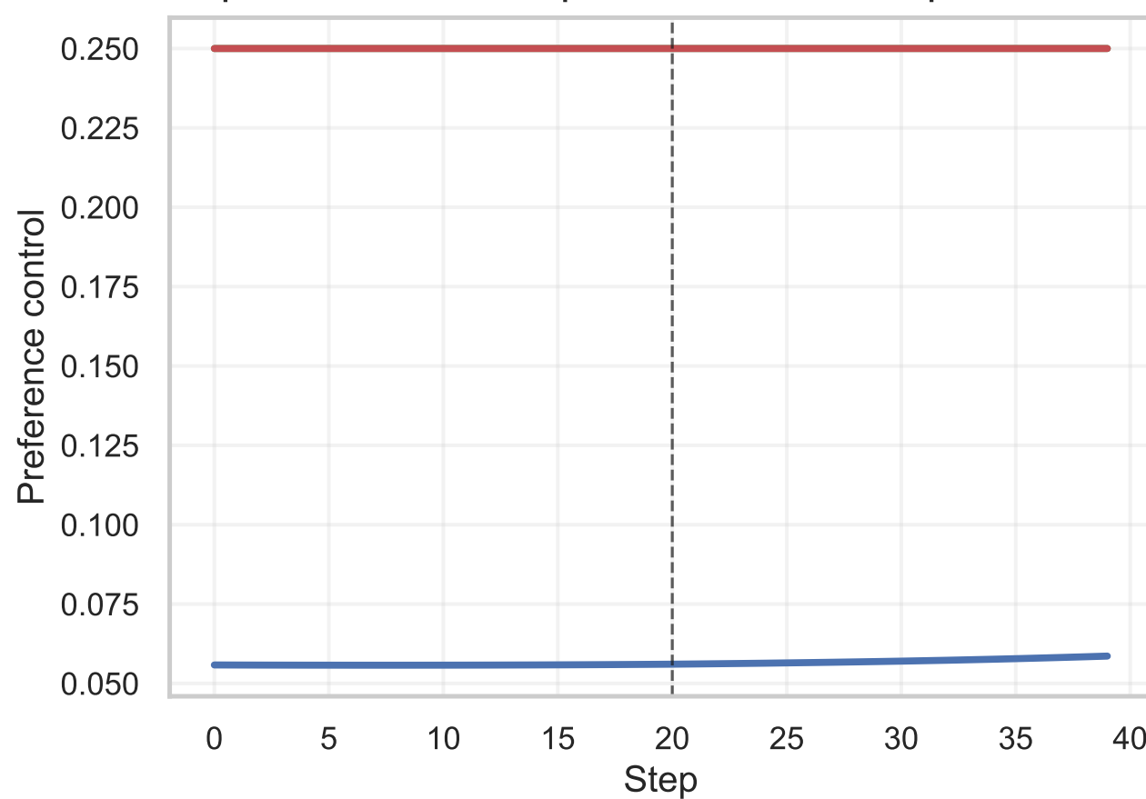
Experiment I: mean preference-control path
