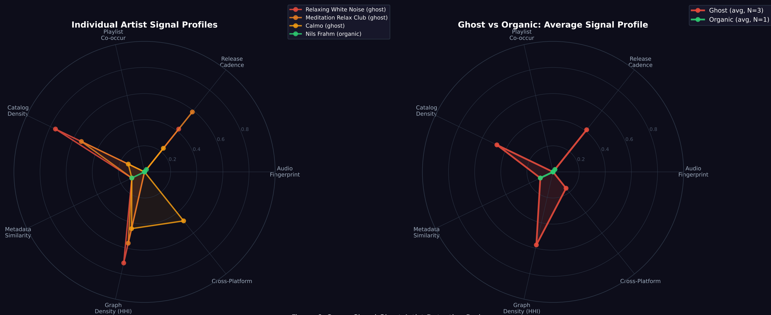
Figure 6: Seven-Signal Ghost Artist Detection Radar Cadence (S2), Catalog Density (S4), and Graph/HHI (S6) most discriminative — Cross-Platform (S7) inconclusive for relaxation genre
