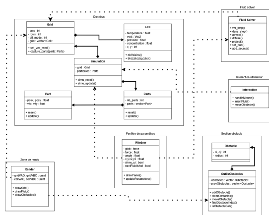
FIGURE 1 – Diagramme UML
