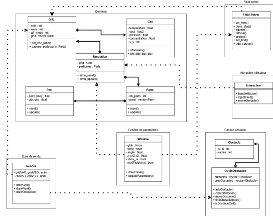
Figure 5: Diagramme UML
