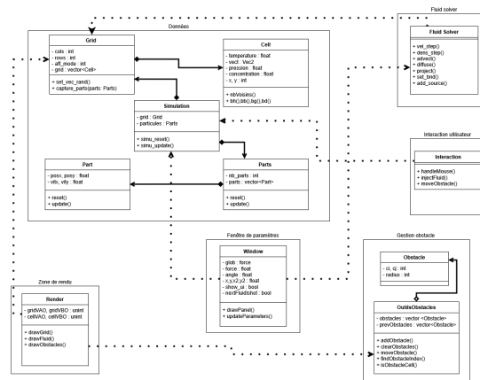
FIGURE 5 – Diagramme UML
