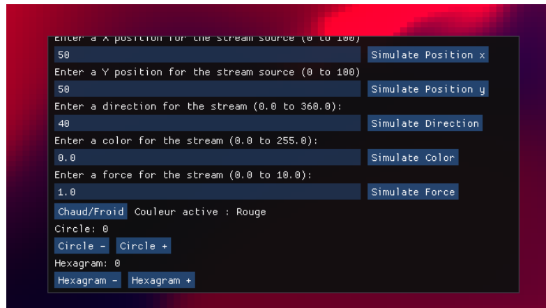
Figure 7: Bouton Chaud/Froid
