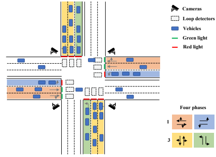
Fig. 1: Illustration of the TSC problem for isolated intersection
