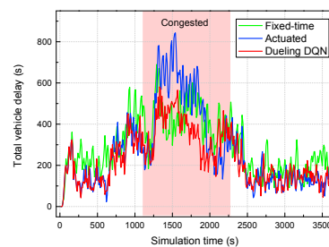
Fig. 3: Total vehicle delay of Dueling DQN and benchmarks
