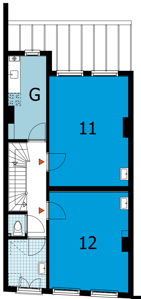
1e verdieping 1st floor
