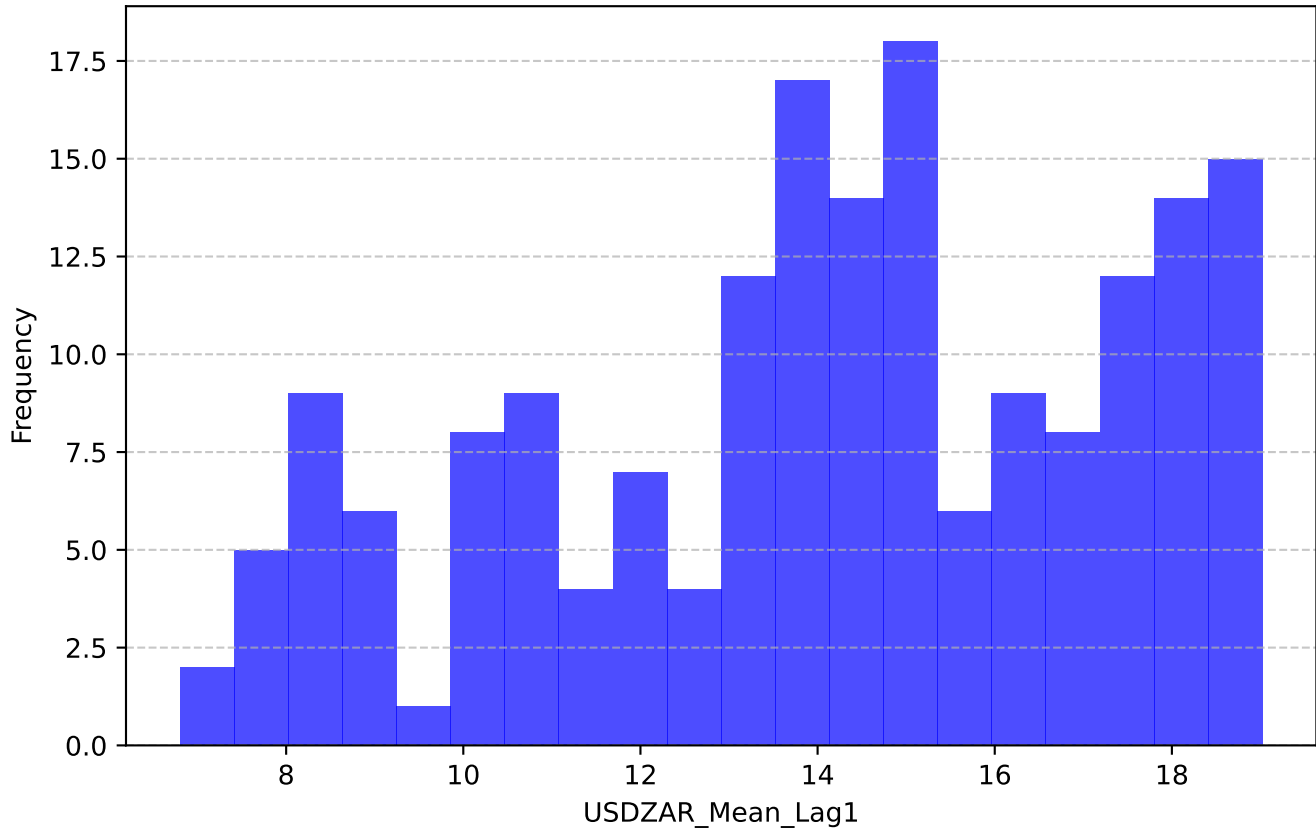
Histogram of USDZAR_Mean_Lag1
