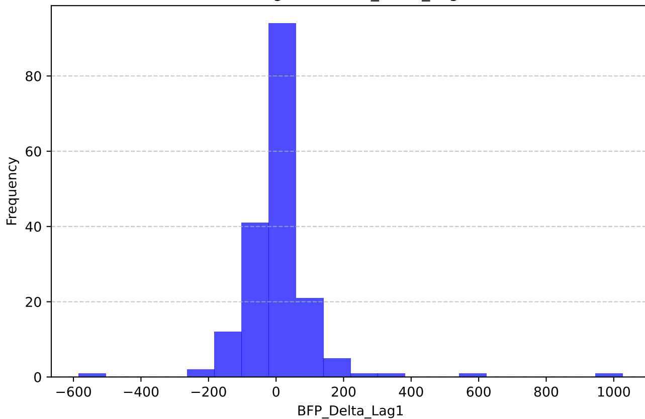
Histogram of BFP_Delta_Lag1
