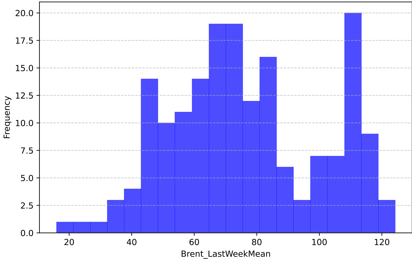
Histogram of Brent_LastWeekMean
