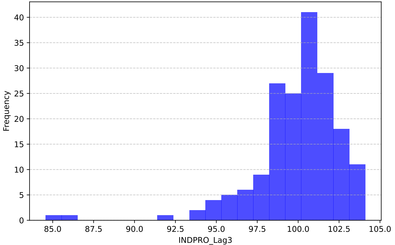
Histogram of INDPRO_Lag3
