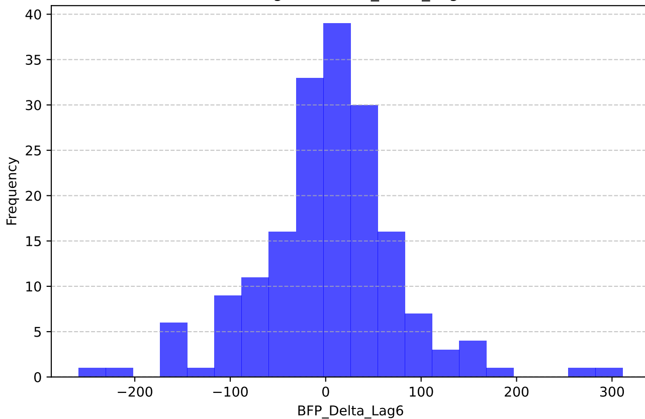
Histogram of BFP_Delta_Lag6
