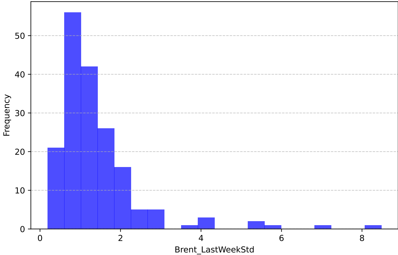
Histogram of Brent_LastWeekStd
