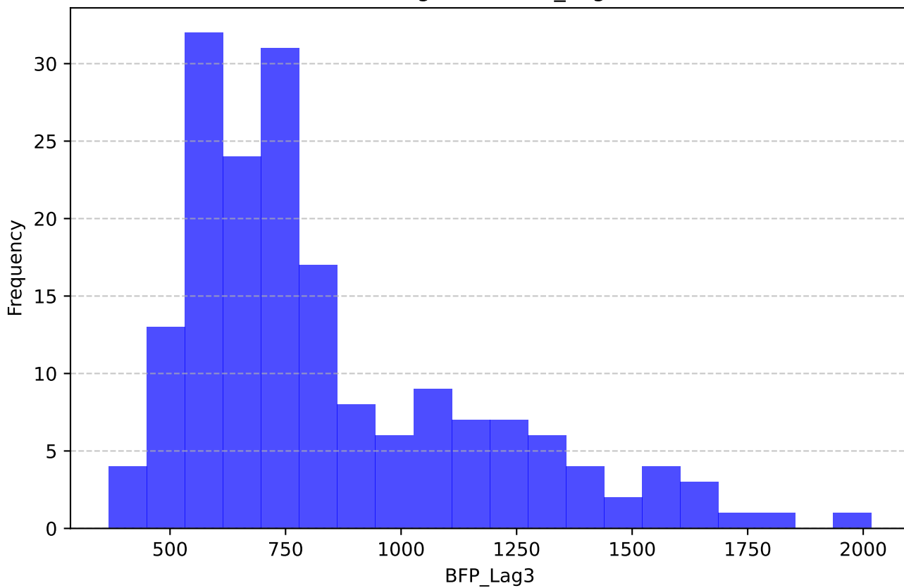
Histogram of BFP_Lag3
