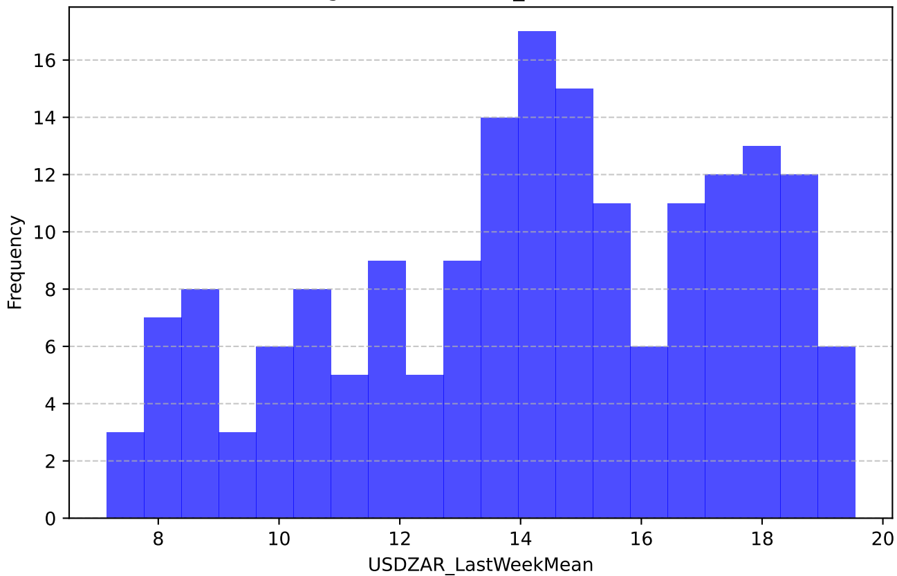
Histogram of USDZAR_LastWeekMean
