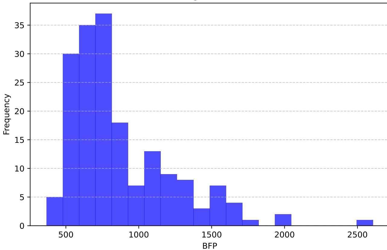
Histogram of BFP
