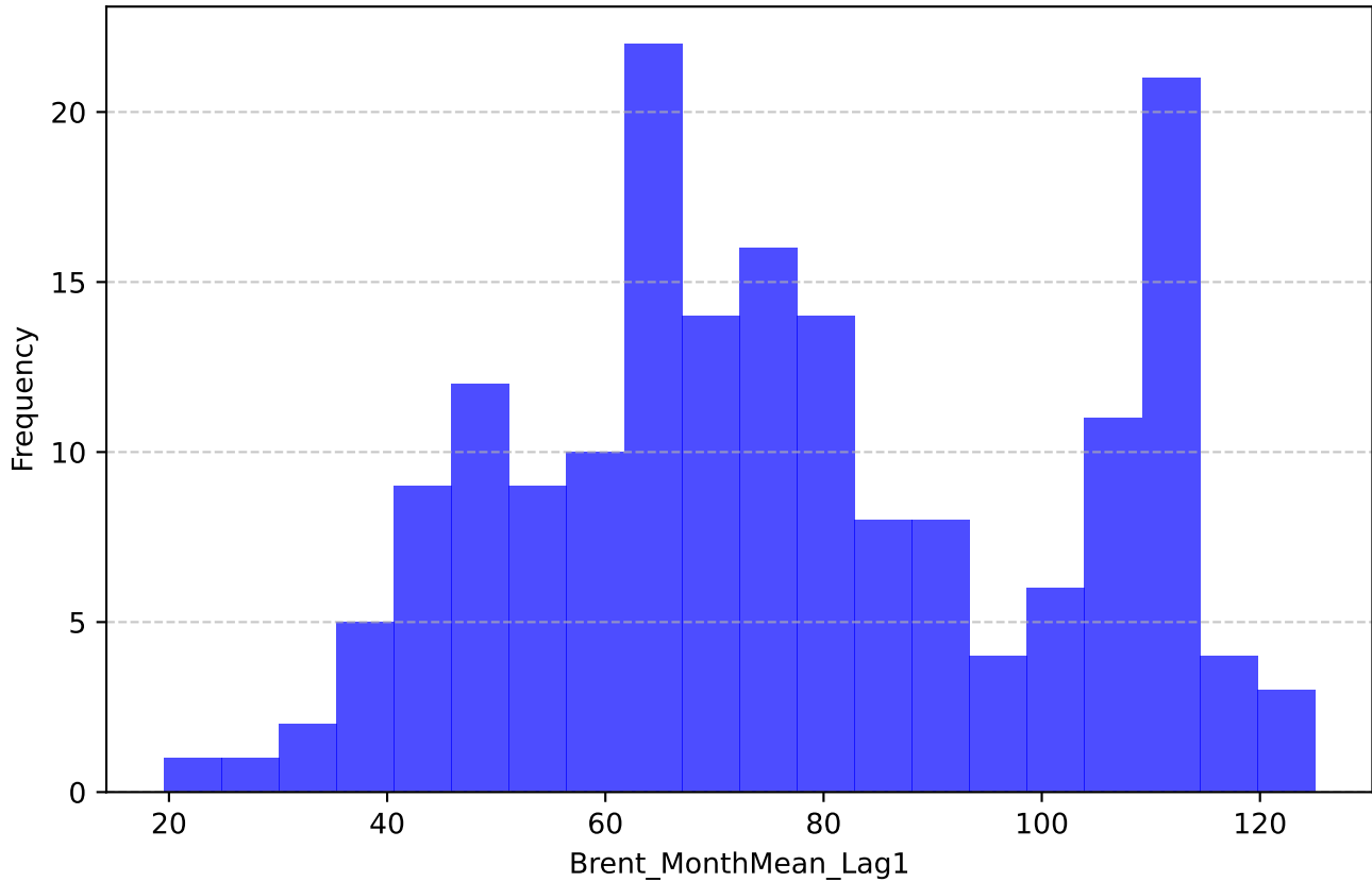
Histogram of Brent_MonthMean_Lag1
