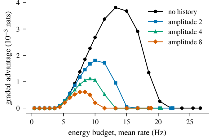
Fig. 2. Under an energy budget the long-window code can be graded below the first count change, but it gains little. Peak count A = 3 (60 Hz, 50 ms windows): advantage of the Blahut–Arimoto optimum over the best binary code on a 0.5 Hz grid, for a neuron without spike history and refractory amplitudes a = 2, 4, 8 ( \tau = 4 ms); zero means that no graded code was shown. The maximizer of the normal approximation was binary in every case.
