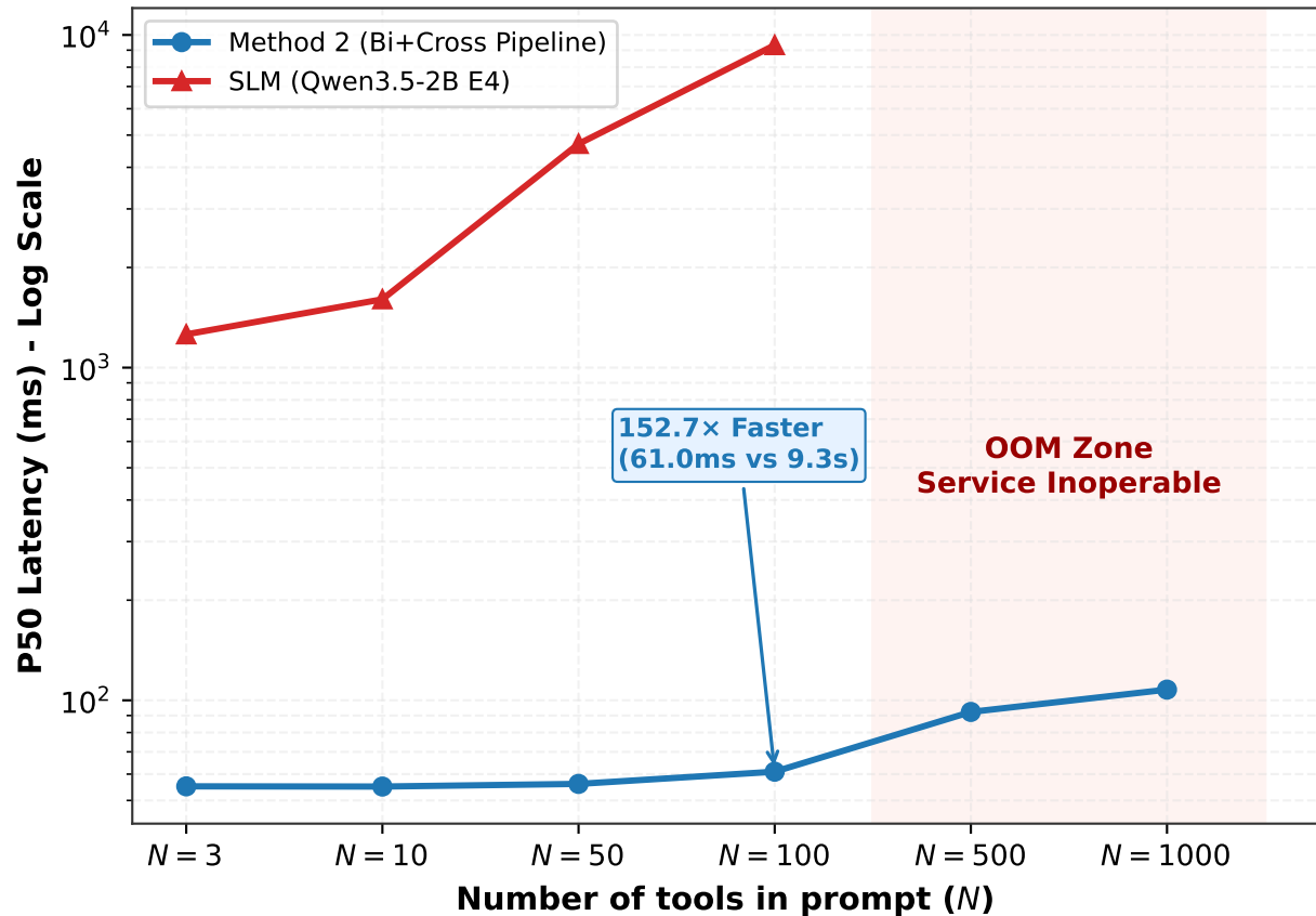
(b) P50 Inference Latency (ms) vs. Tool Scale
