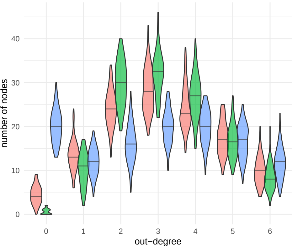
Out-degree distribution across 100 simulated networks
