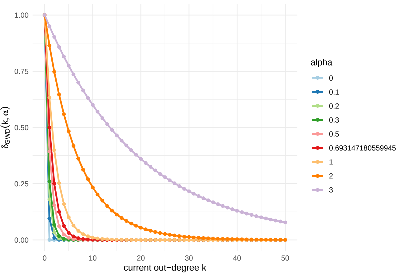
Change statistic for non.negative decay values
