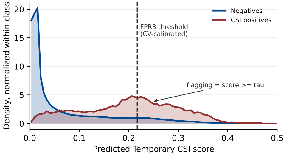
TEST scores by true label
