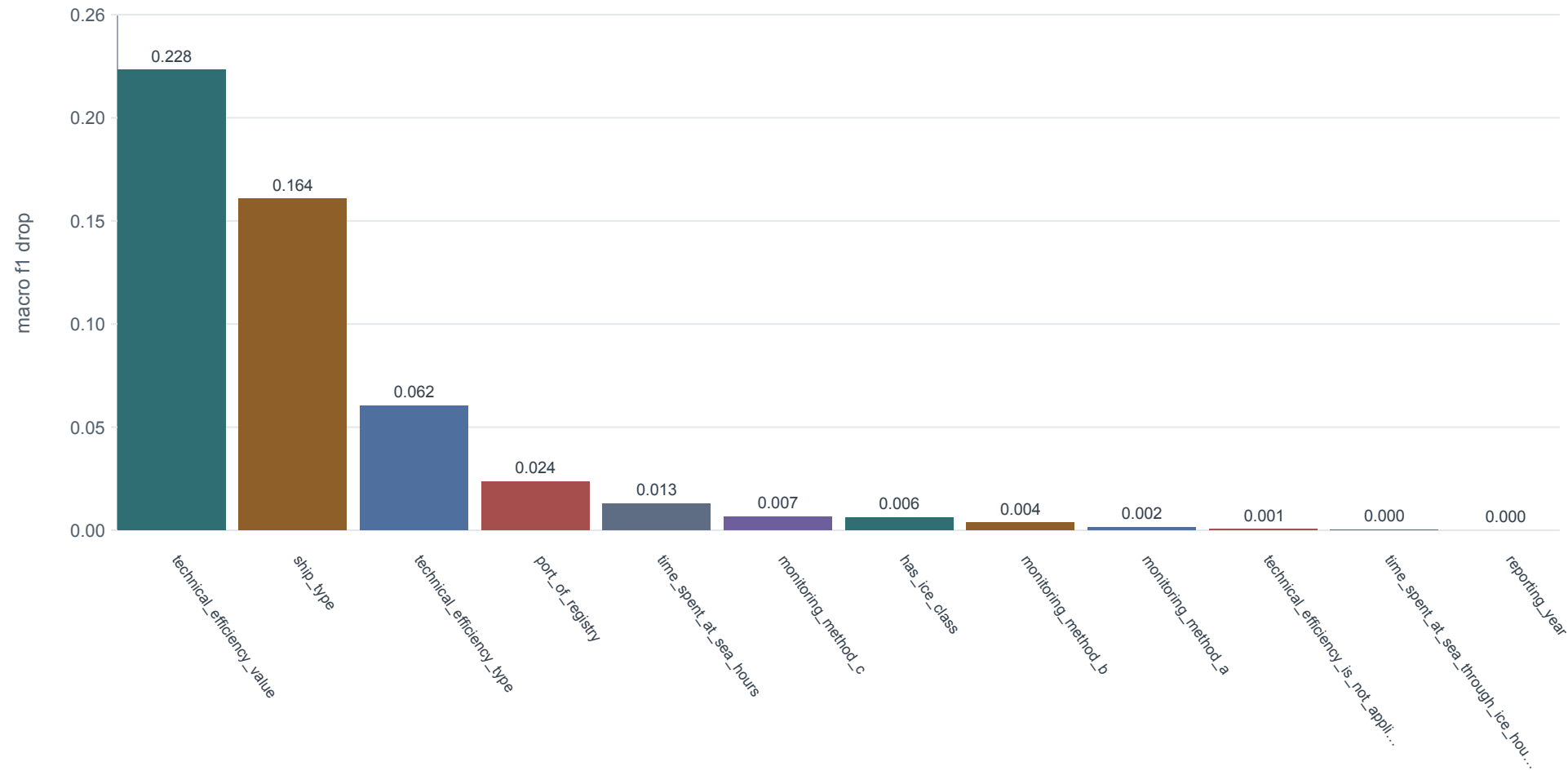
Permutation importance: Macro-F1 drop
