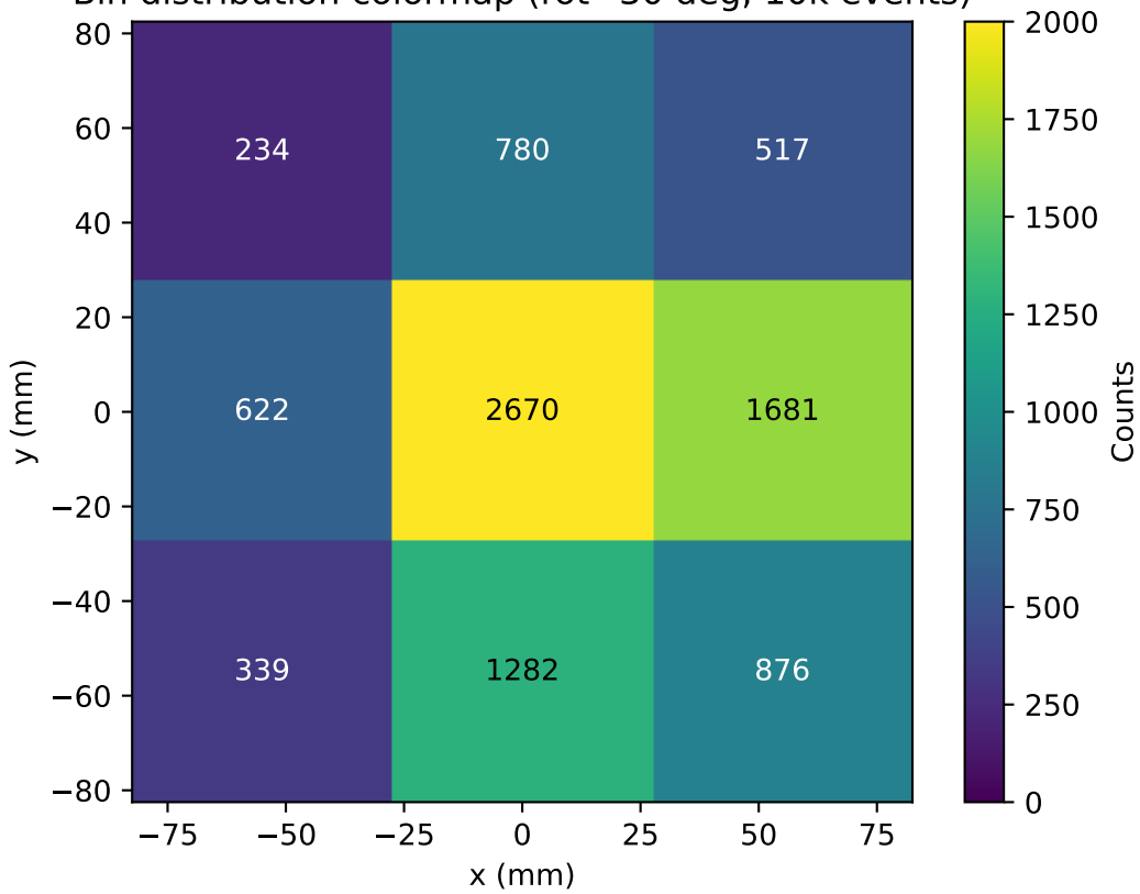
Bin distribution colormap (rot=30 deg, 10k events)
