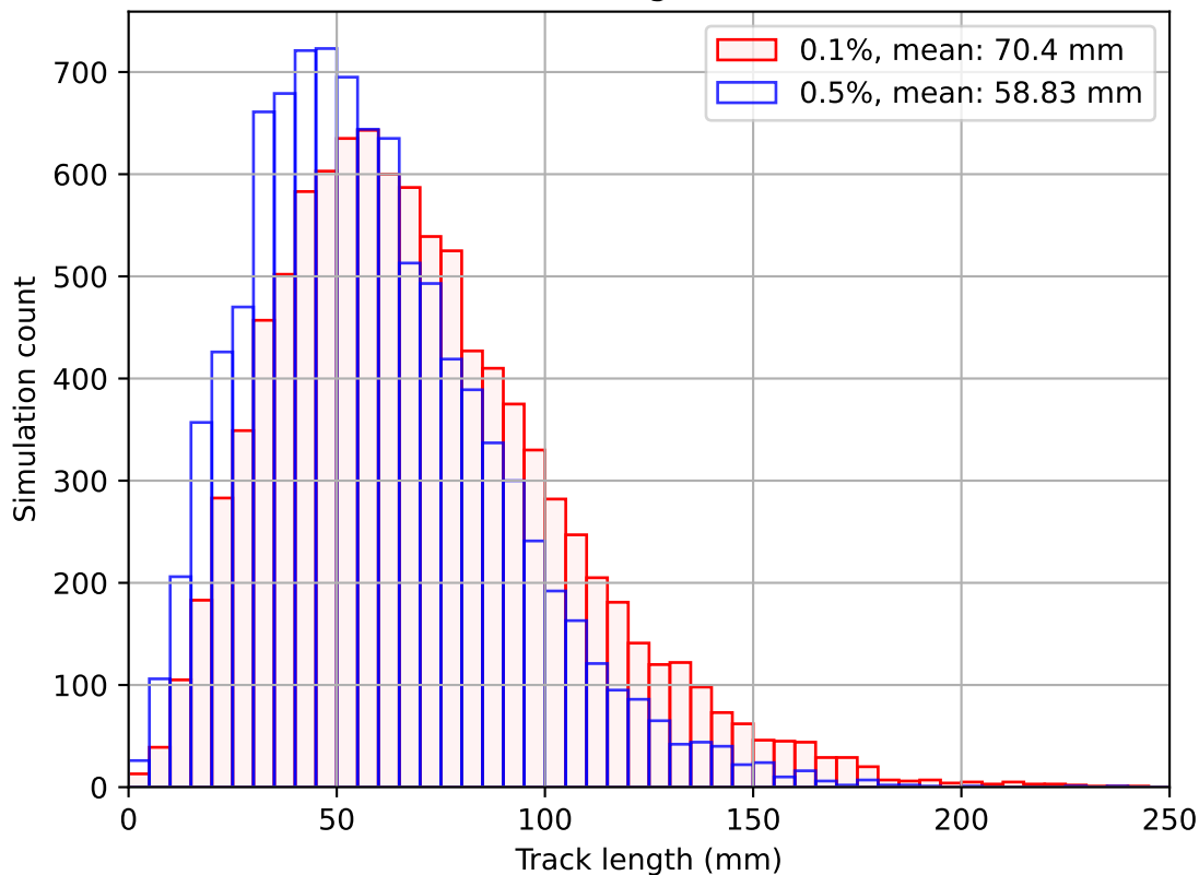
Neutron track lengths (10k events)
