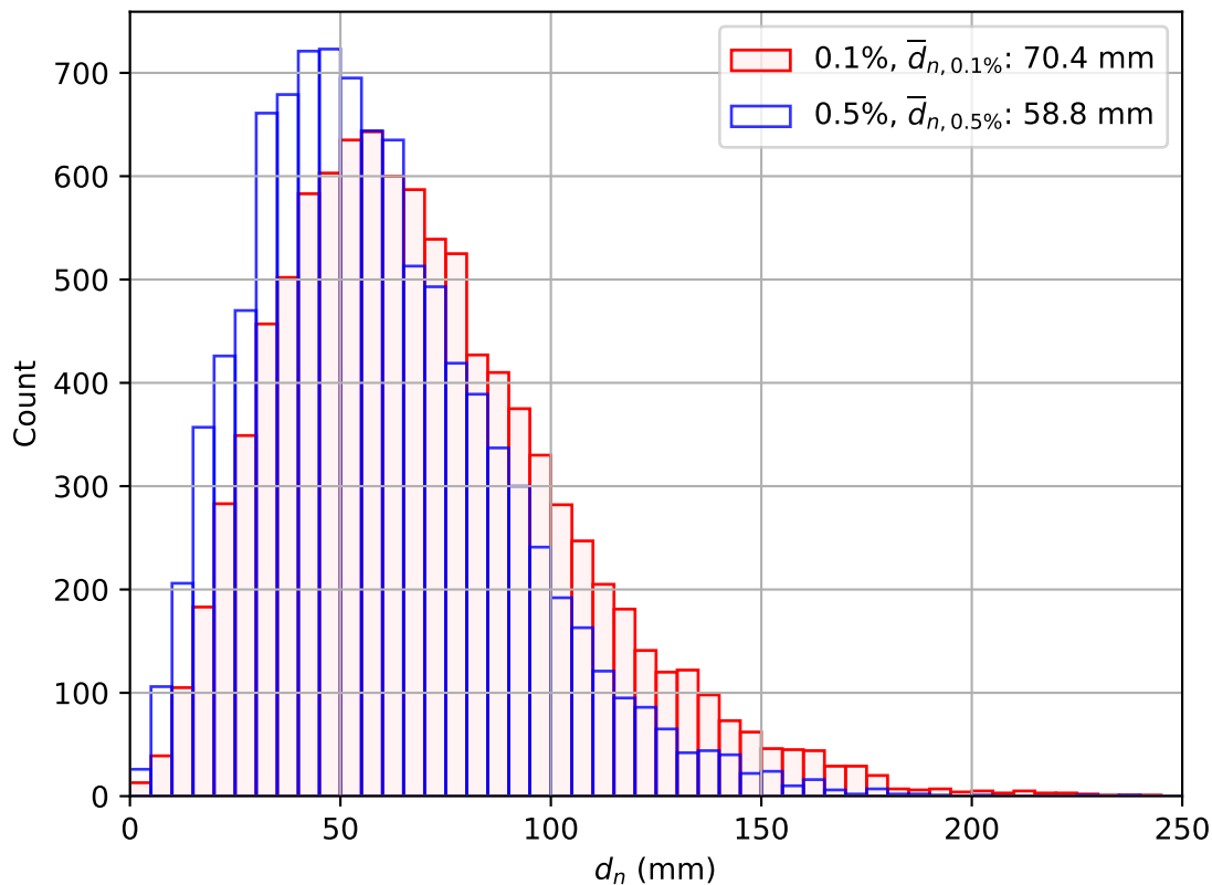
Neutron path length distribution ( d_n , 10k events)
