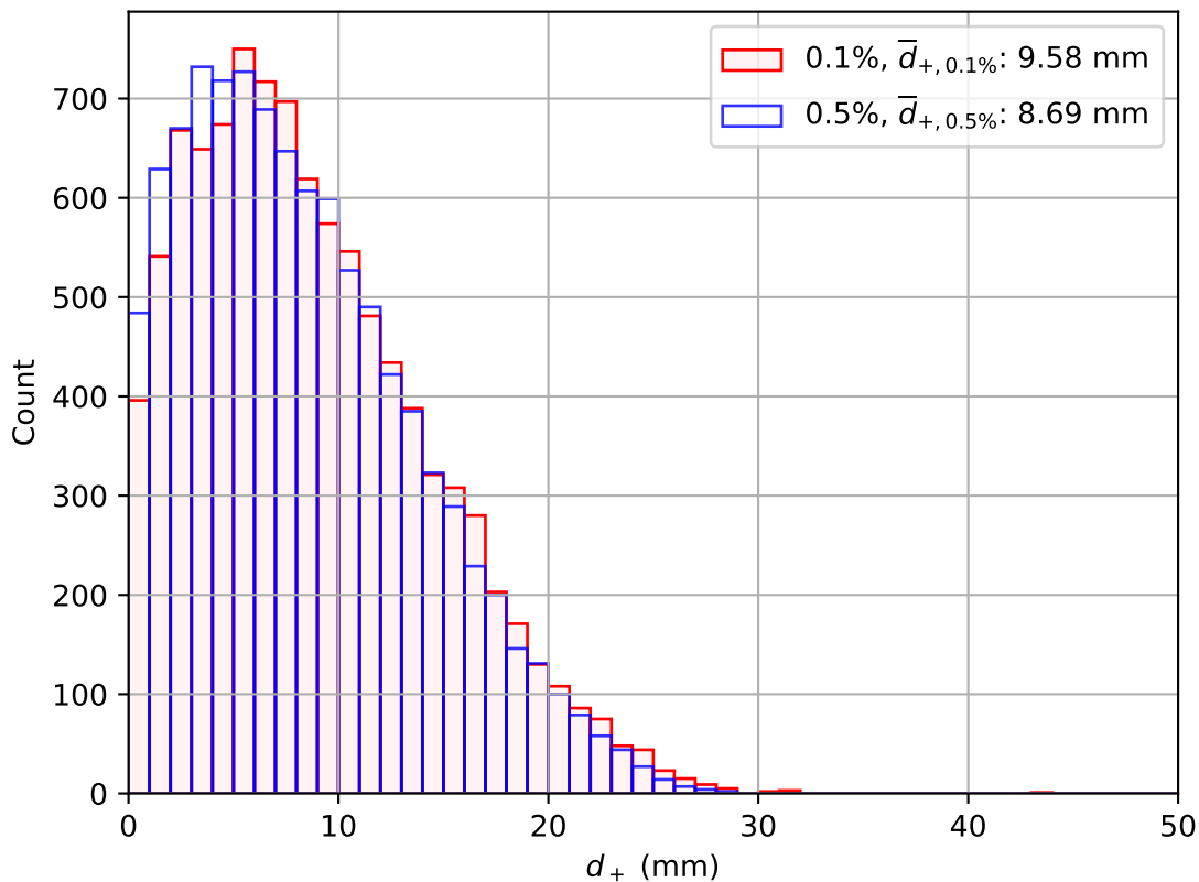
Positron path length distribution ( d_+ , 10k events)
