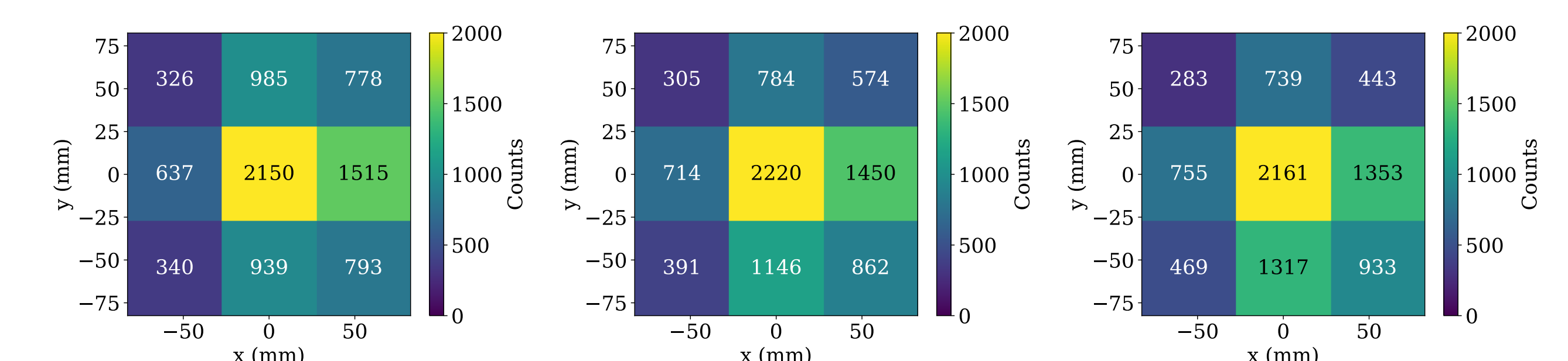
Figure 5: Examples of binning distributions for incoming angles \vartheta_\nu = 0^\circ, -30^\circ, -45^\circ , 0.1% ^6\text{Li} -doped. The direction of antineutrinos is indicated by the arrows below the plots.
