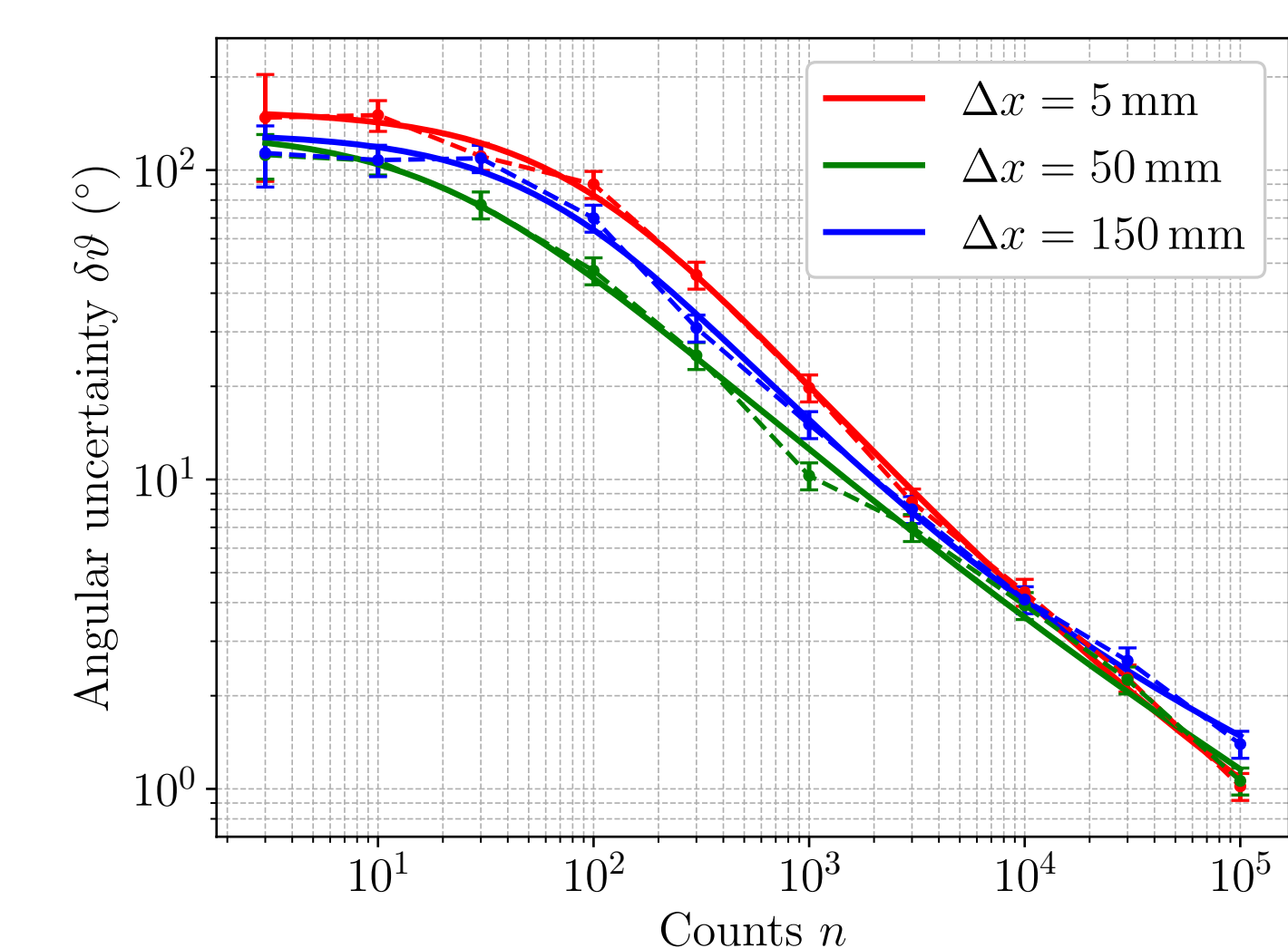
Figure 7: Angular uncertainty plot comparing the performance of three different square segment sizes: 5 mm, 50 mm and 150 mm.
