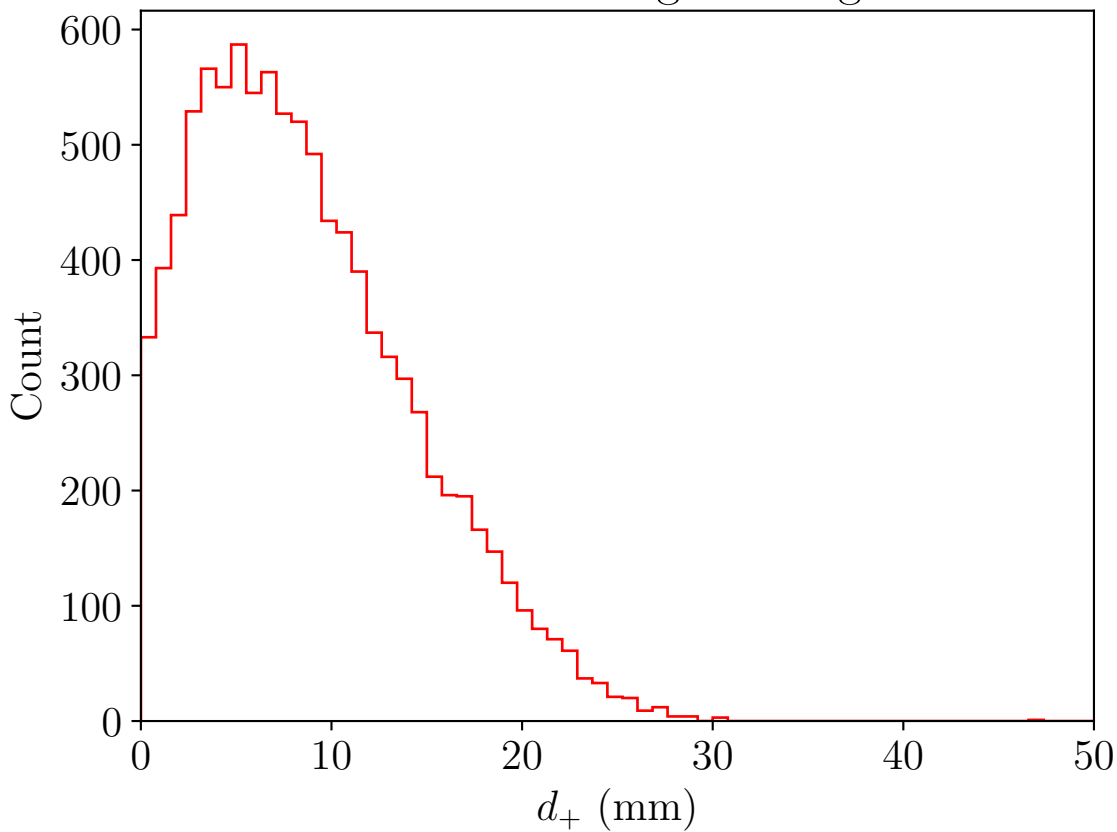
Positron track length histogram
