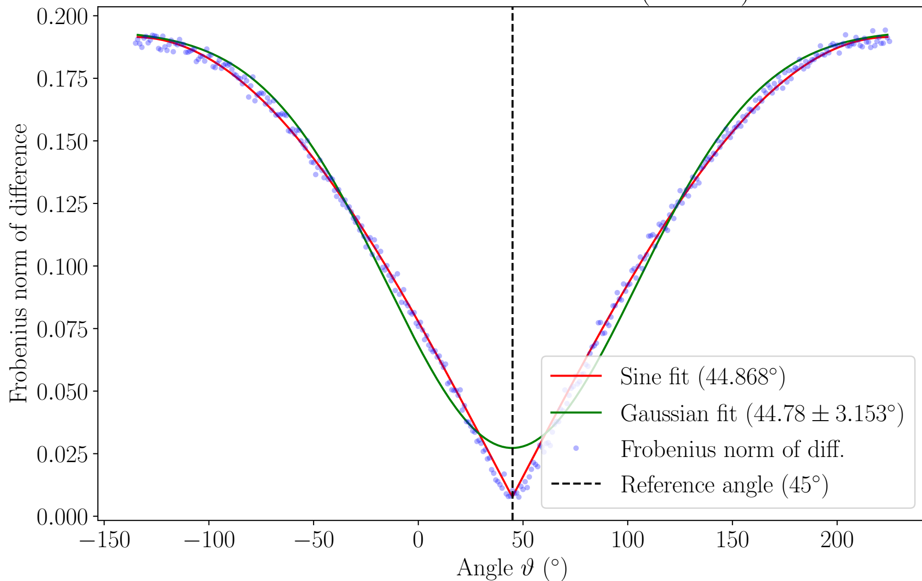
Frobenius norms of differences ( \theta = 45^\circ )
