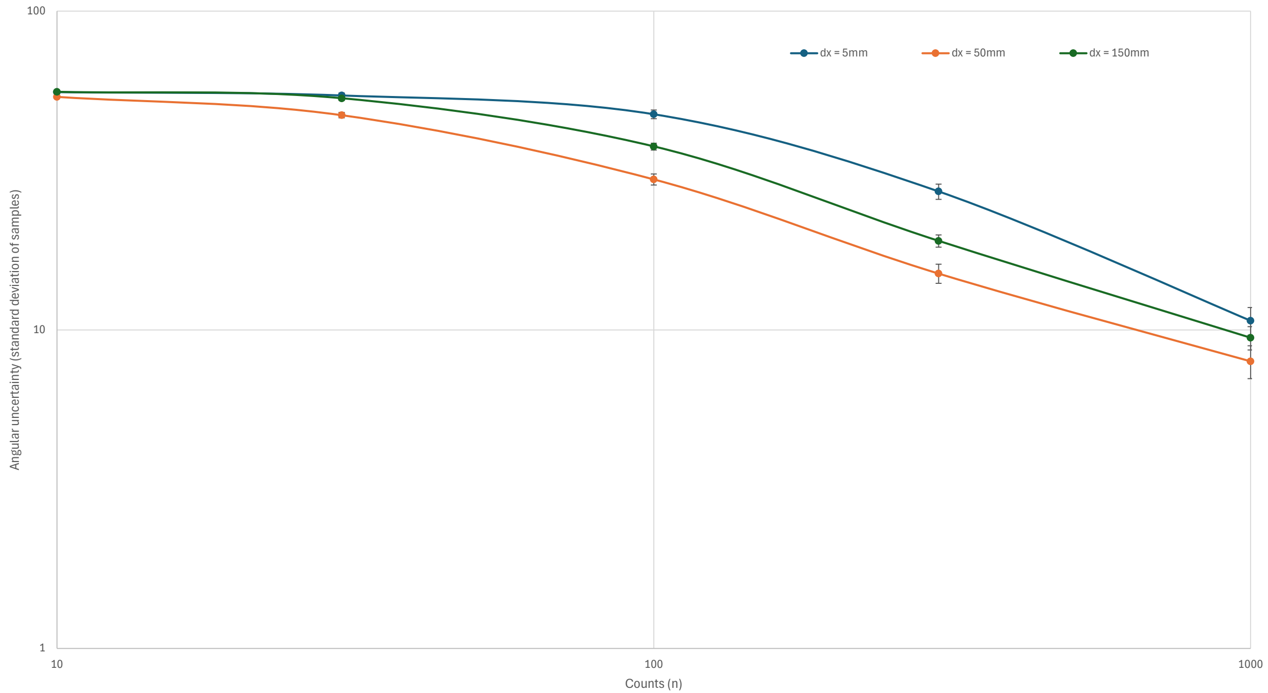
Angular uncertainty test using RATPAC2 data
