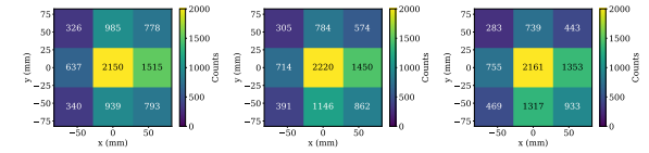
Figure 5: Examples of binning distributions for incoming angles \theta_\nu = 0^\circ, -30^\circ, -45^\circ , 0.1% ^6\text{Li} -doped. The direction of antineutrinos is indicated by the arrows below the plots.
