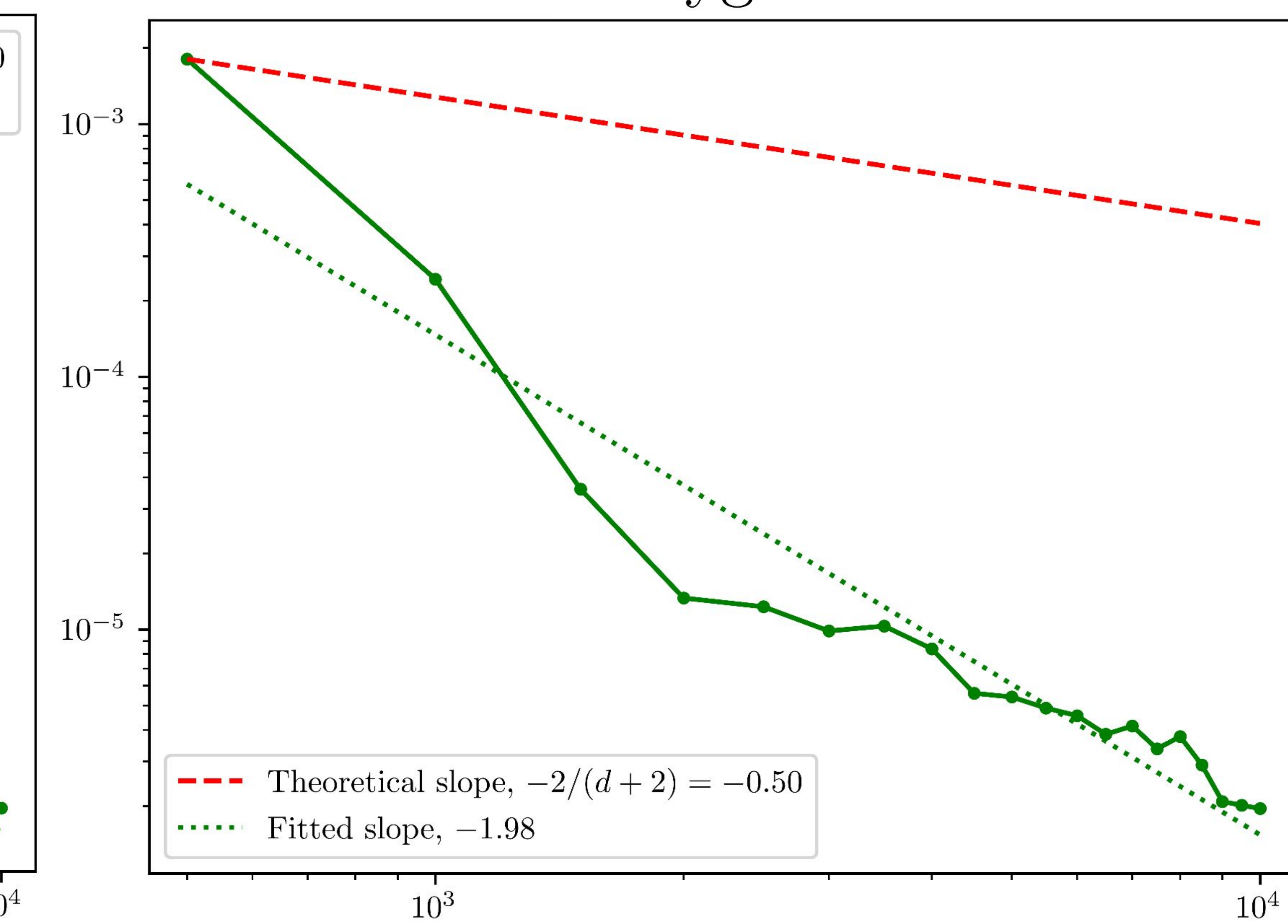
Polygon
