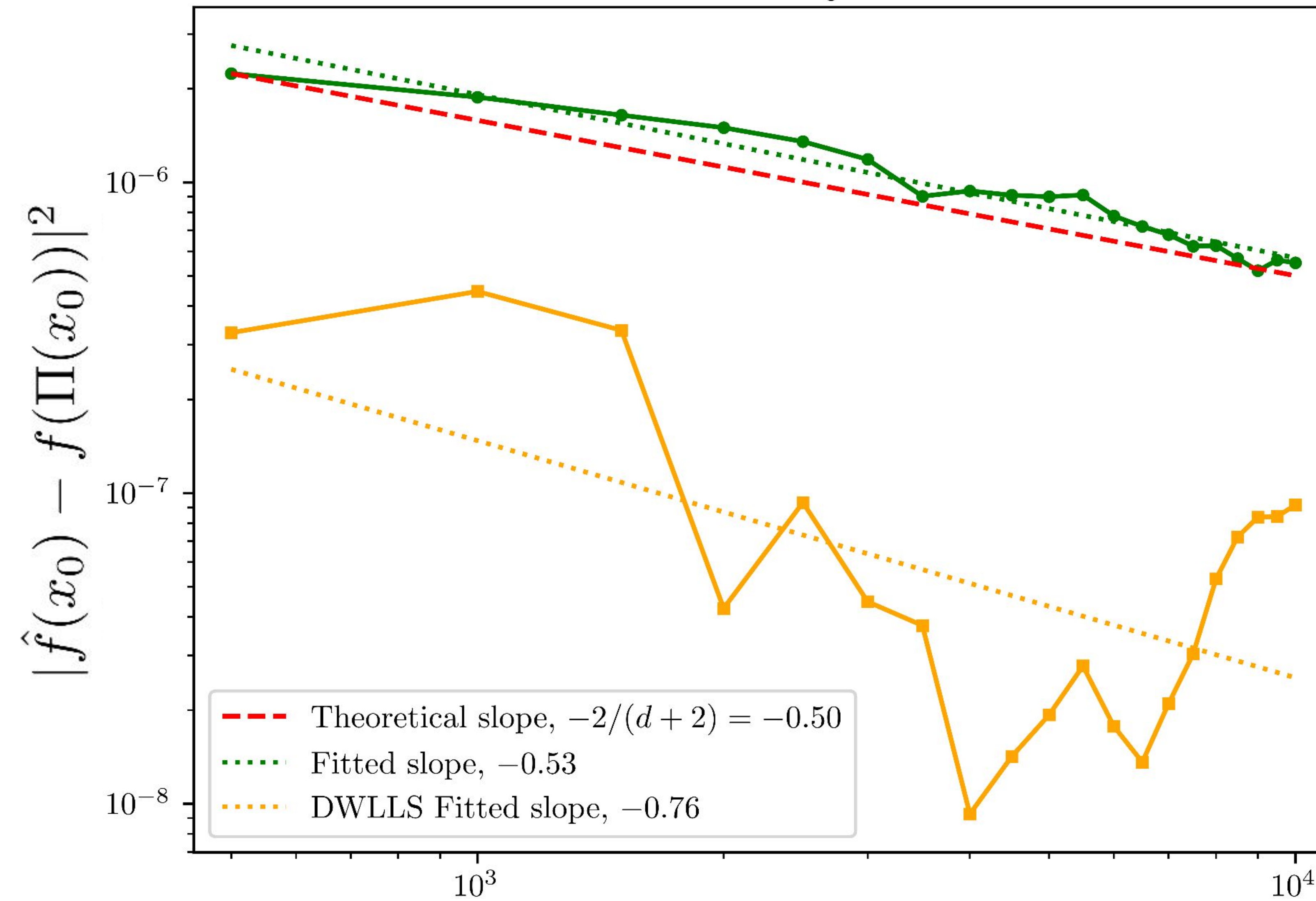
Identity
