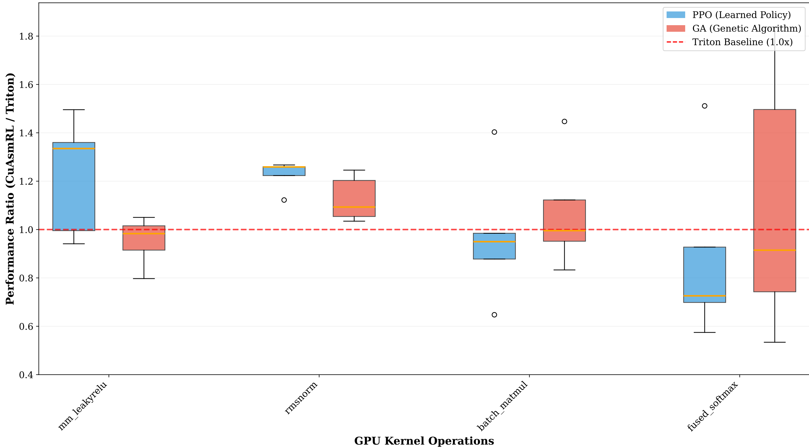
CuAsmRL Performance Comparison: PPO vs GA (Pairwise Relative Performance)
