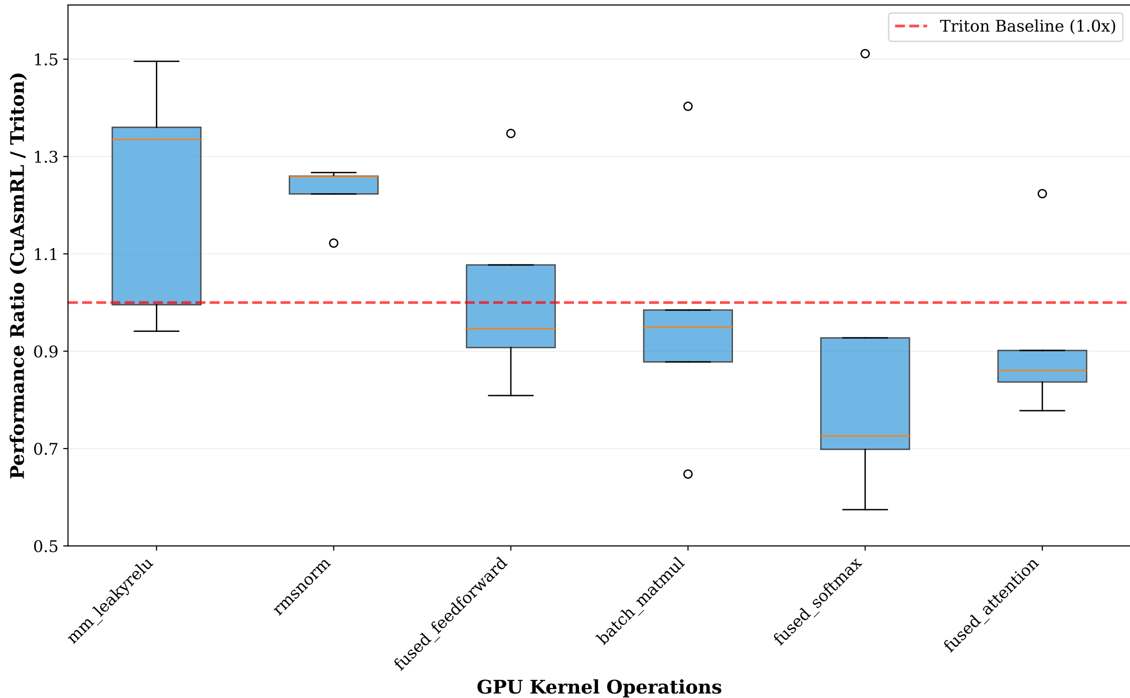
CuAsmRL Performance Variability: Pairwise Comparison Across 5 Runs
