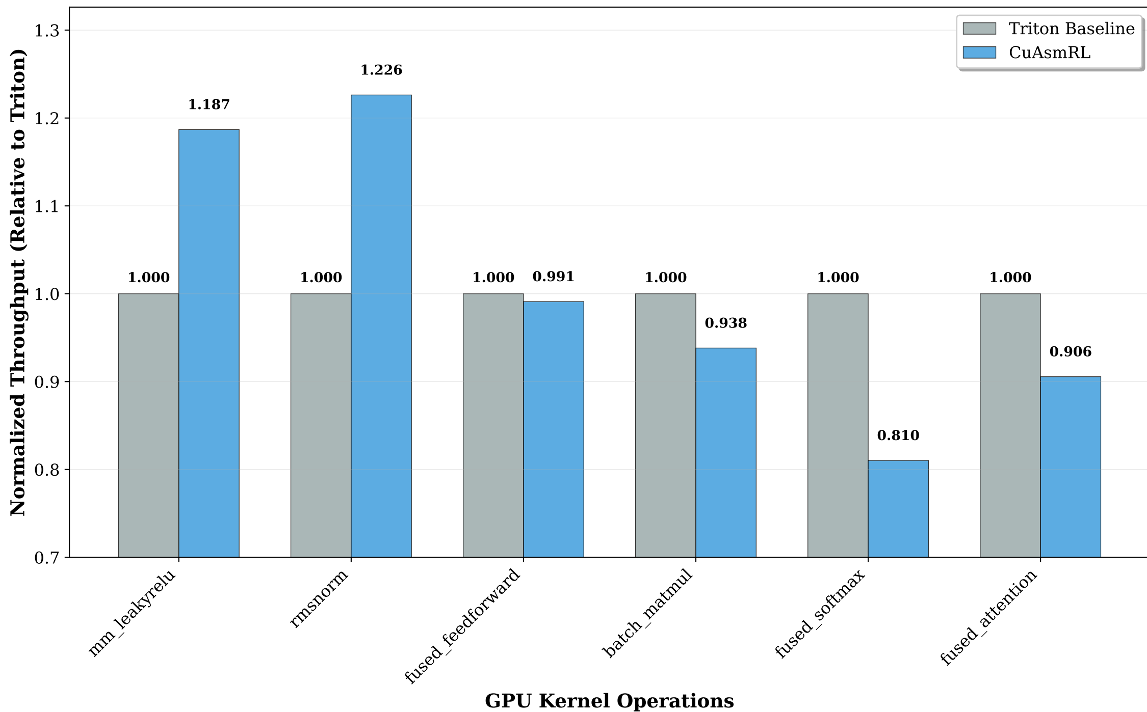
CuAsmRL Performance vs Triton Baseline
