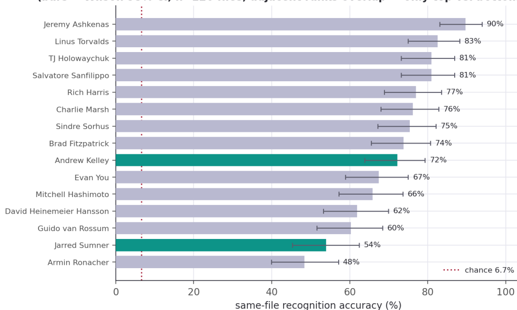
Some developers are far more recognizable than others (bars = Wilson 95% CI, n=126 files; adjacent ranks overlap — only top vs. bottom is separable)
