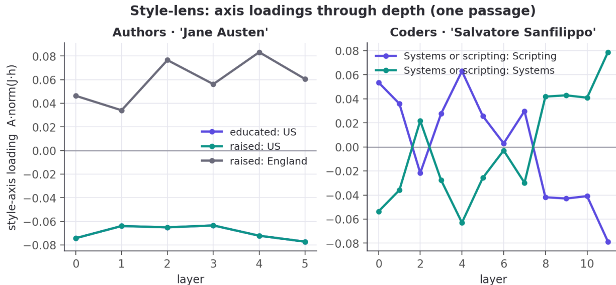
Figure 9: Style-lens axis loadings through depth for one passage.
