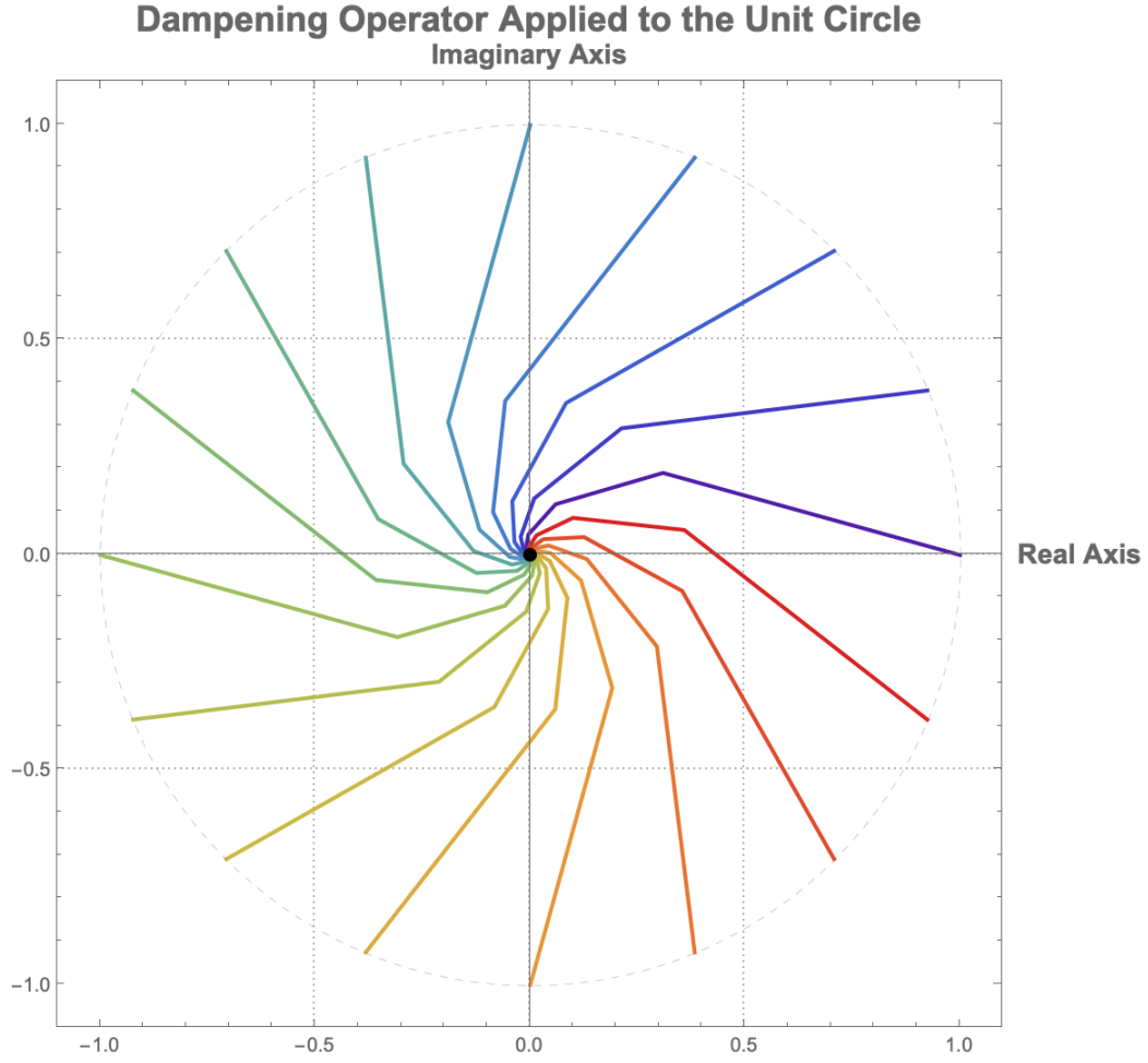
Figure 4: The Dampening Operator ( \Lambda_{G1} ) applied to 16 points on the unit circle. Regardless of the starting angle, every path spirals inward, demonstrating the operator's universal converging property.
