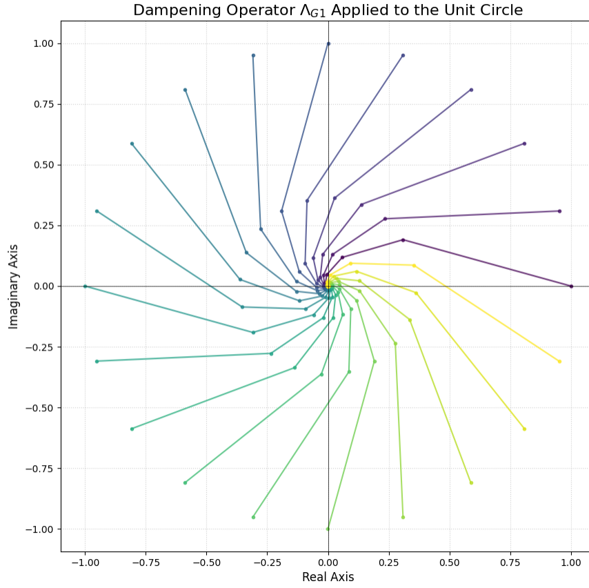
Figure 2: The action of the Dampening Operator \Lambda_{G1} on points originating on the unit circle. All trajectories converge to the origin, visually demonstrating the inherent stability of the framework's core operator.
